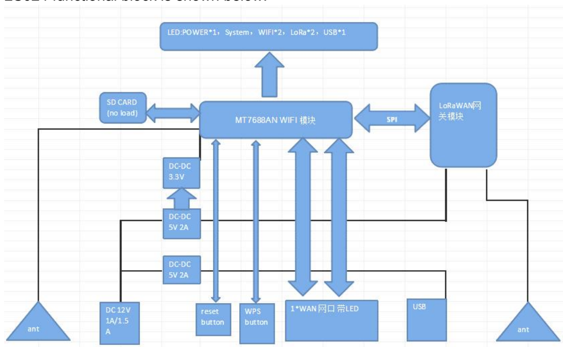
Figure 2- 1 RHF2S024 functional block
