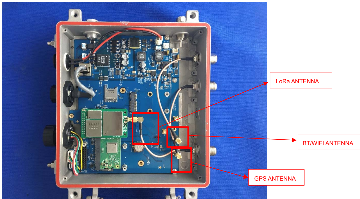
EUT UNCOVER VIEW
