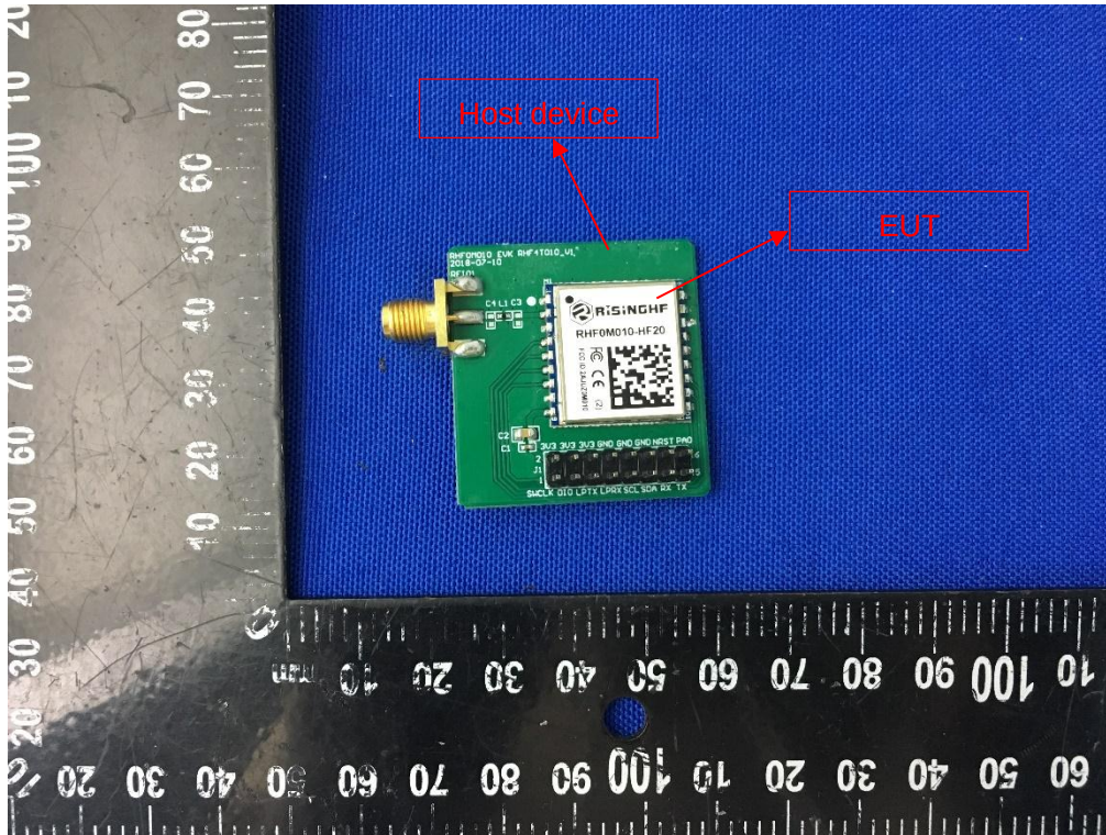
TOP VIEW OF EUT (WITH HOST DEVICE)
