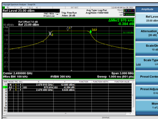
LoRa(812kHz) HIGH CHANNEL
