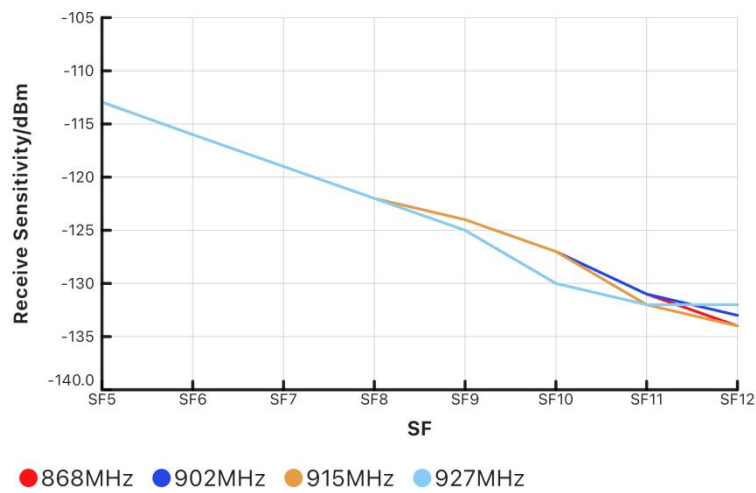
Figure 9 RF Receiver Sensitivity vs Spreading factor (868~927MH@BW125KHz)
