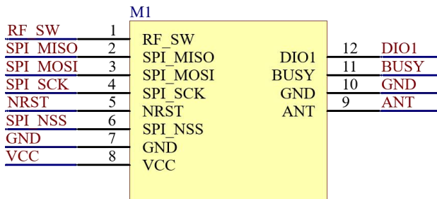
Figure 2 RHF0M62H Pin arrangement
