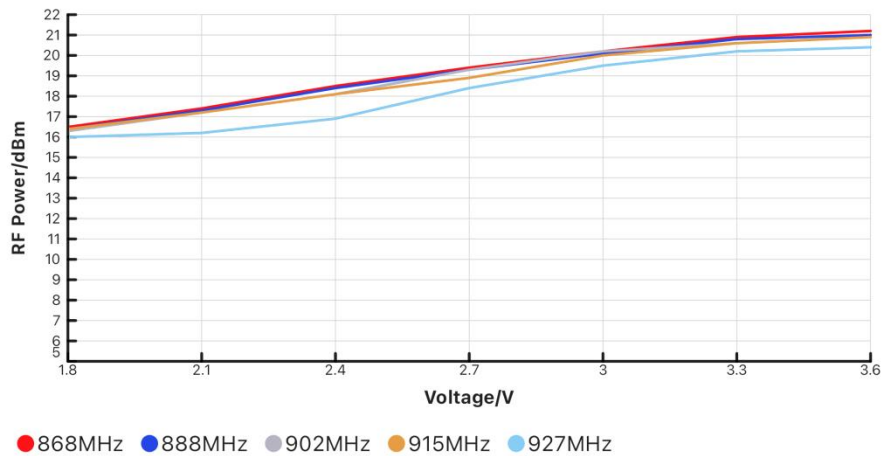
Figure 7 Max RF Power vs Voltage (868~927MHz)
