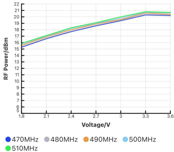
Figure 3 Max RF Power vs Voltage (470~510MHz)
