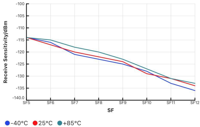
Figure 6 RF Receiver Sensitivity VS Temperature (470MHz@BW125KHz)
