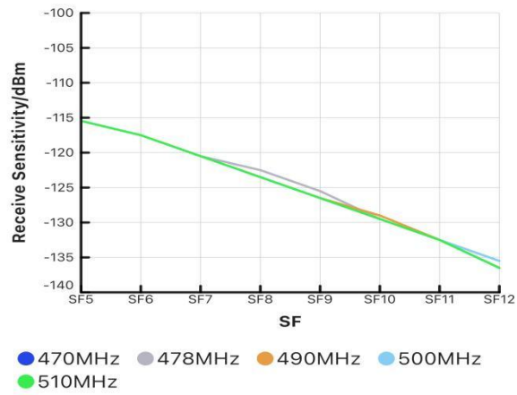
Figure 5 RF Receiver Sensitivity vs Spreading factor (470~510MHz@BW125KHz)
