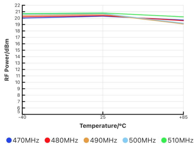
Figure 4 Max RF Power VS Temperature (470~510MHz)
