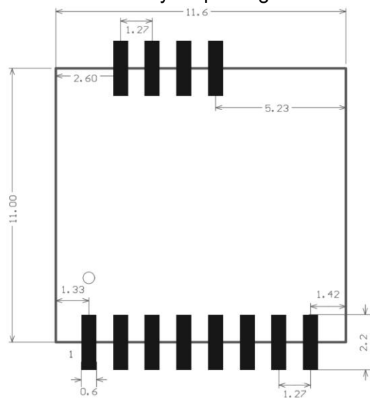
Figure 12 RHF0M62H Module appearance
