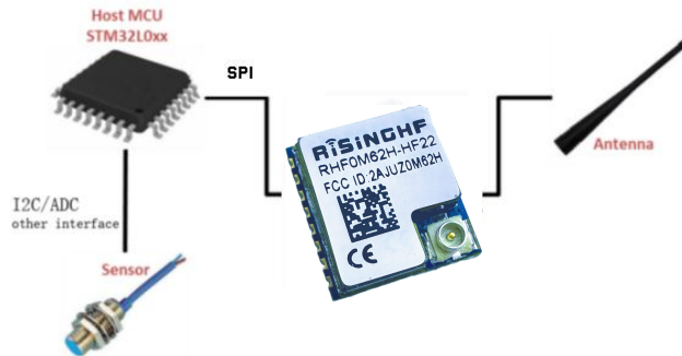
Figure 15 Design of LoRaWAN® wireless sensor based on RHF0M62H module
