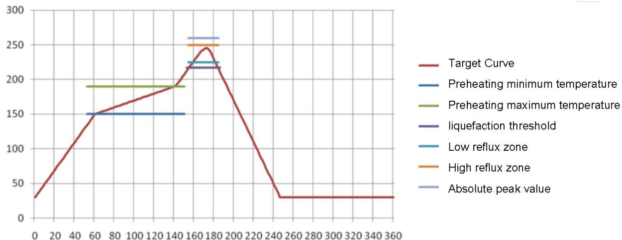
Figure 16 Reflow profile
