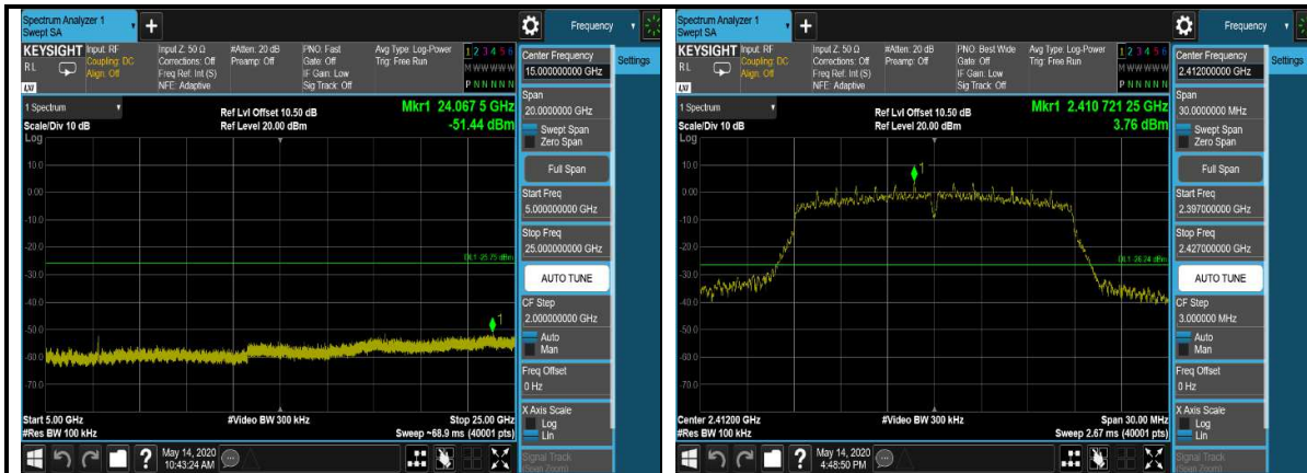
802.11n(HT20),2412MHz,Ant1,Plot 2,Band Edge
