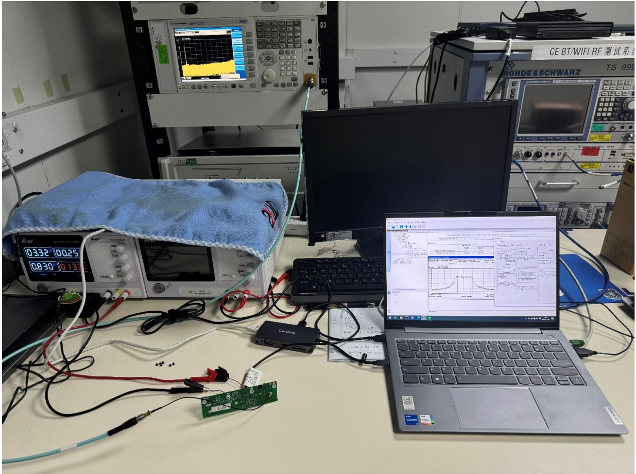
RF Conducted Test setup (WIFI)
