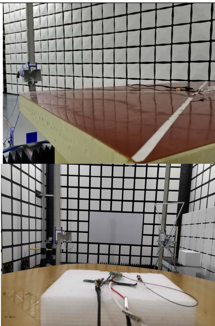
Spurious Radiated Emissions Test setup
