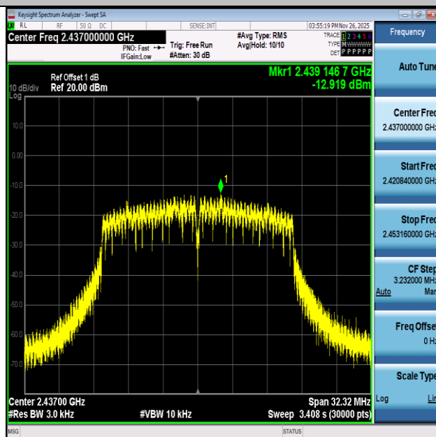
11N20ISO-Ant1-2437-PASS
