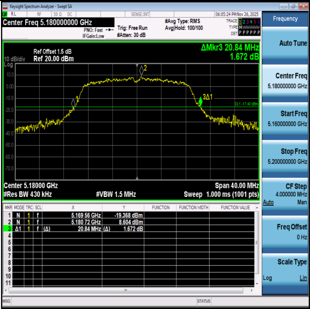
11N20SISO-Ant1-5180
