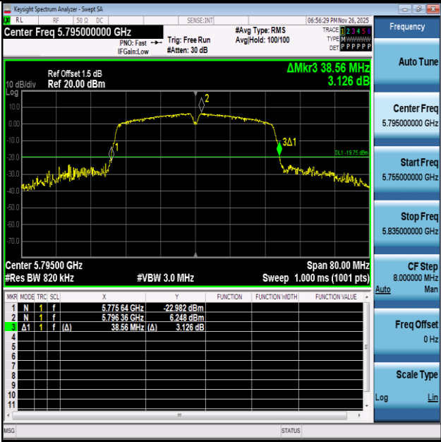
11N40SI50-Ant1-5795
