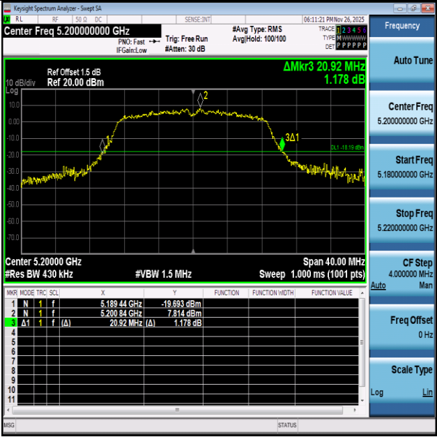
11N20SISO-Ant1-5200
