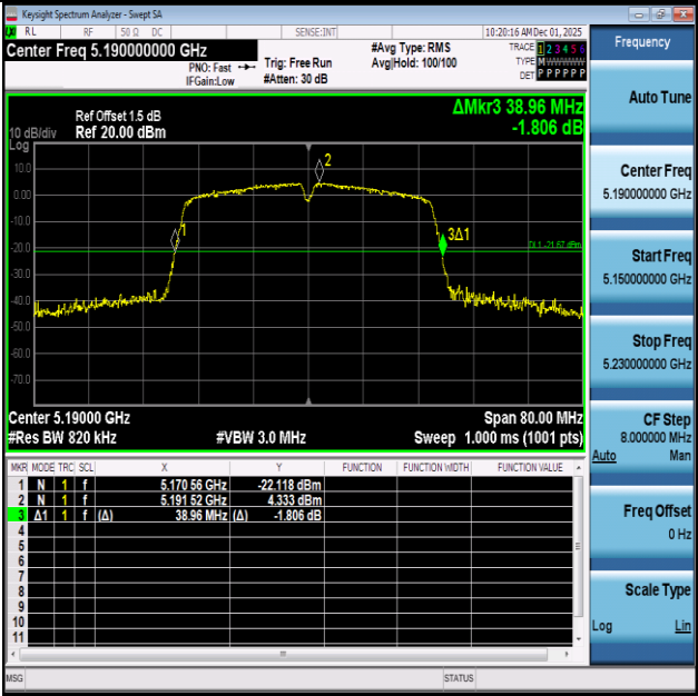
11N40SISO-Ant1-5190
