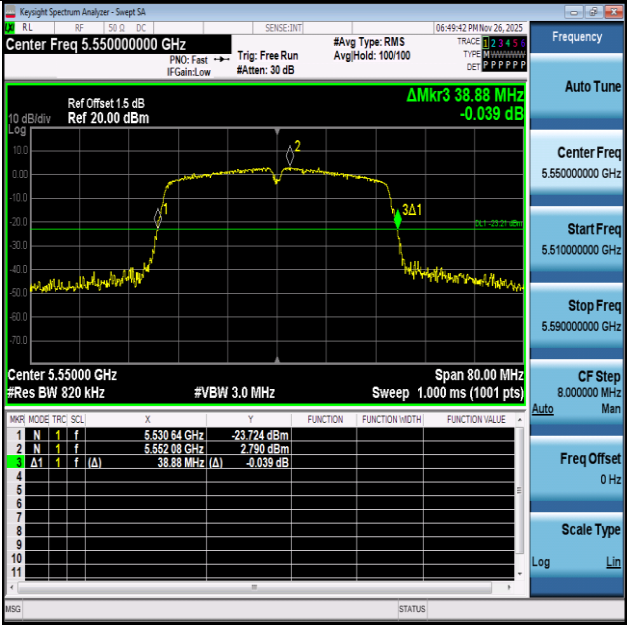
11N40SISO-Ant1-5550
