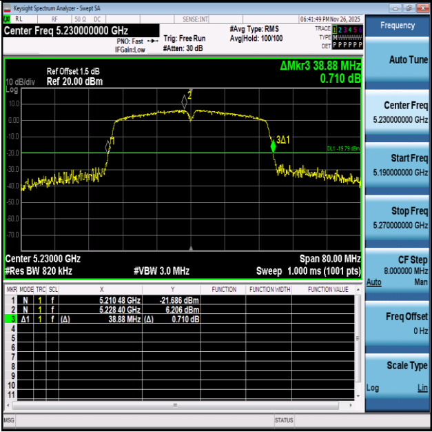
11N40SISO-Ant1-5230
