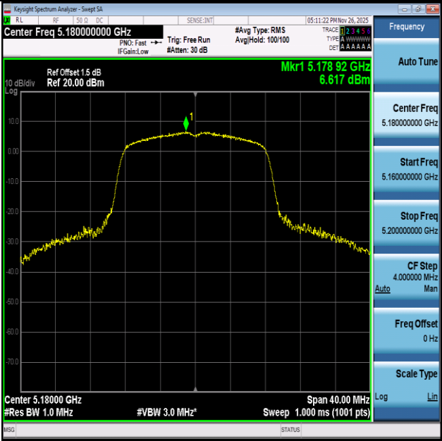
11A-Ant1-5180-PASS
