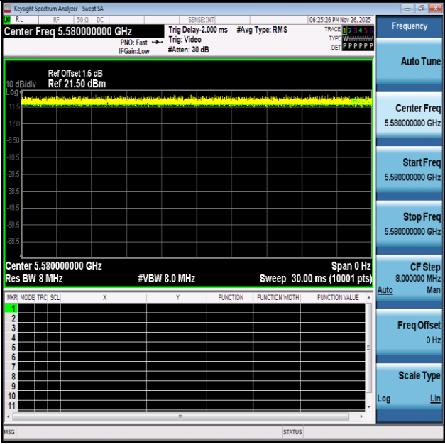
NTNV-11N20SISO-Ant1-5580
