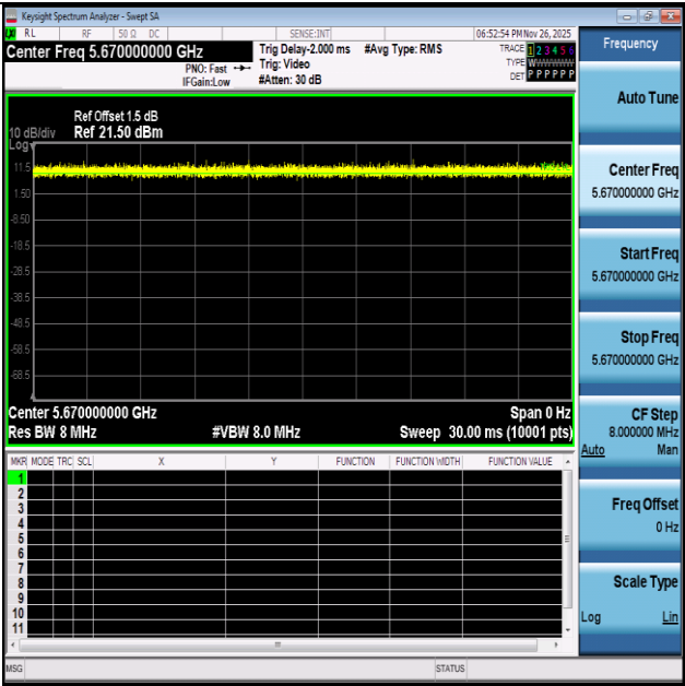
NTNV-11N40SISO-Ant1-5670
