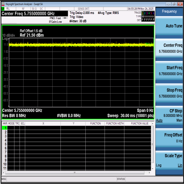
NTNV-11N40SISO-Ant1-5755
