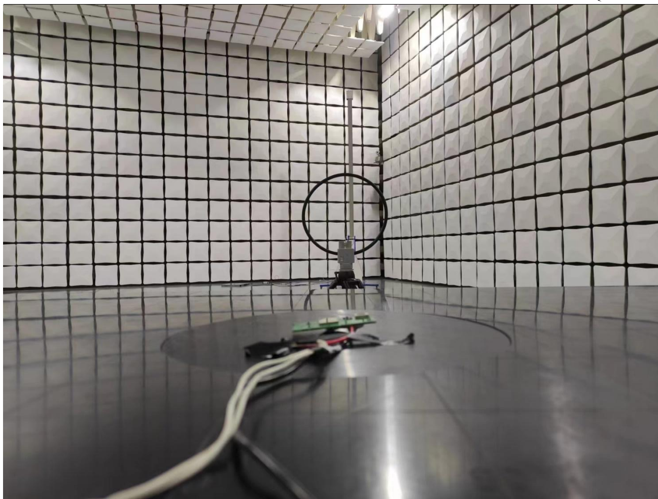
RE 9KHz~30MHz
