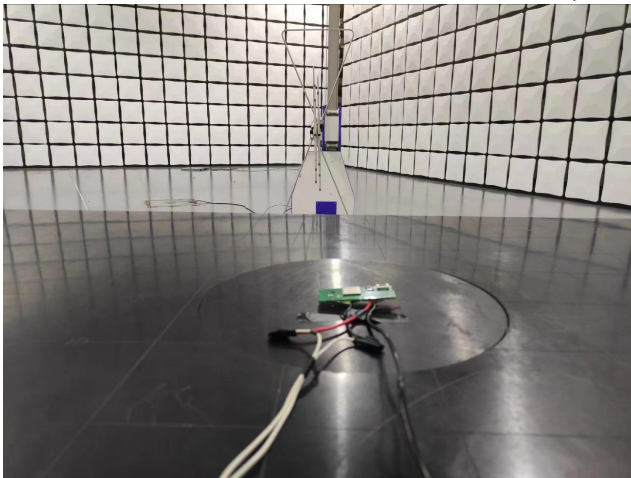
RE 30MHz~1GHz
