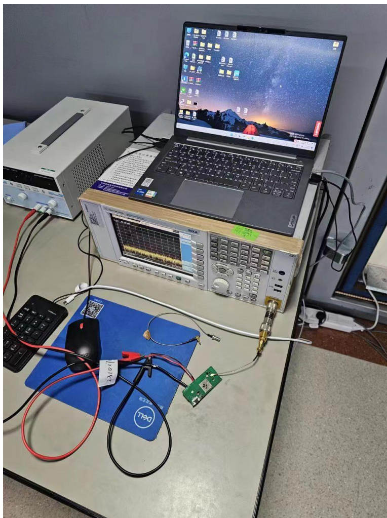
RF Conducted Test setup (BT/WIFI)
