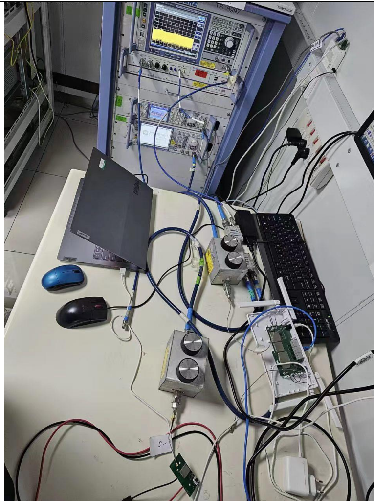
RF Conducted Test setup (DFS)
