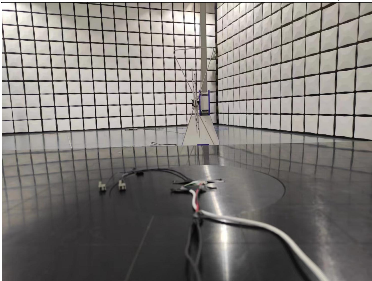
RE30MHz~1GHz
