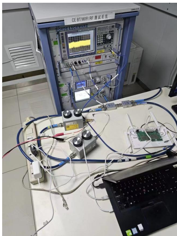
RF Conducted Test setup (DFS)
