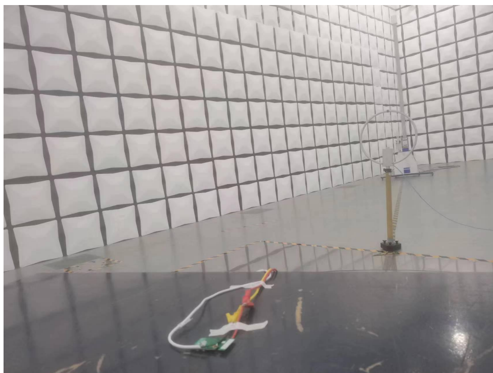
RE 9KHz~30MHz
