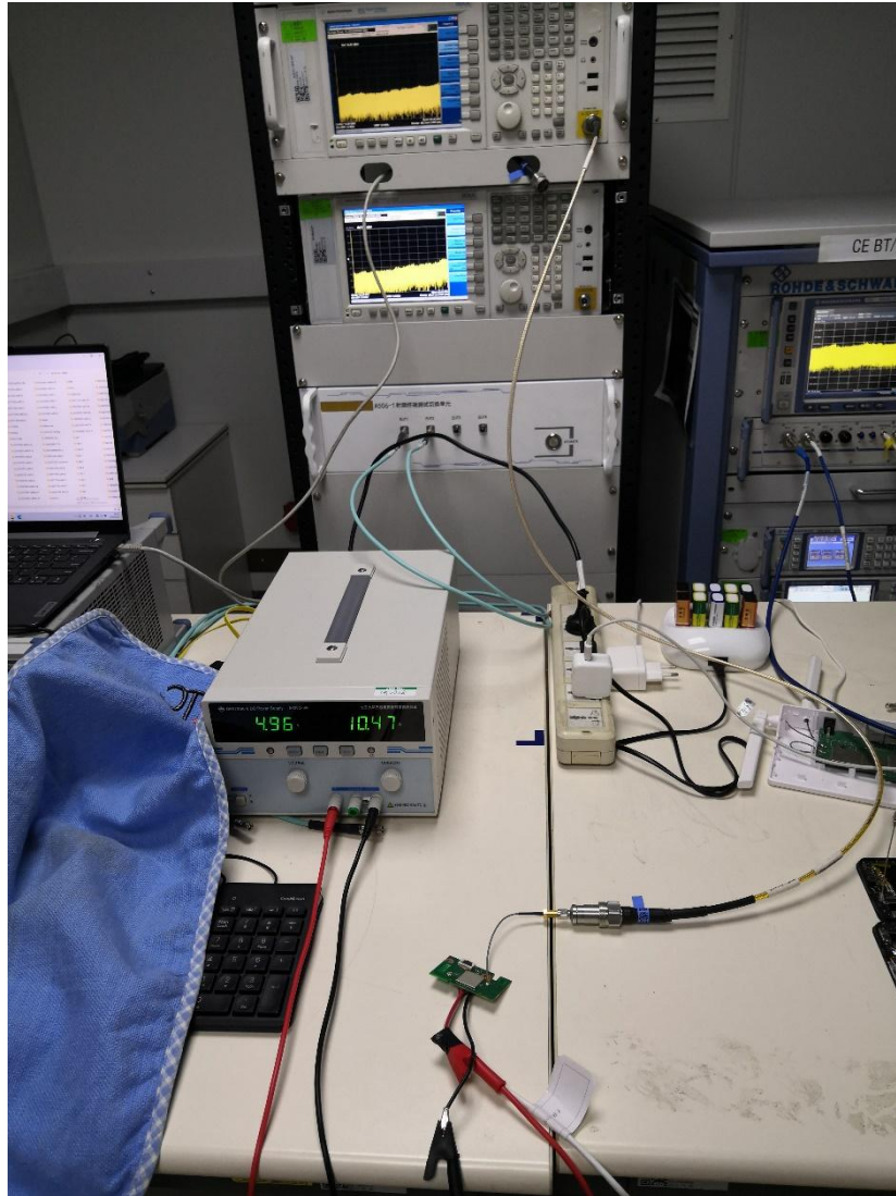
RF Conducted Test setup (BT/WIFI)
