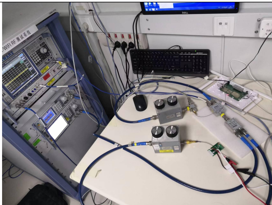
RF Conducted Test setup (DFS)
