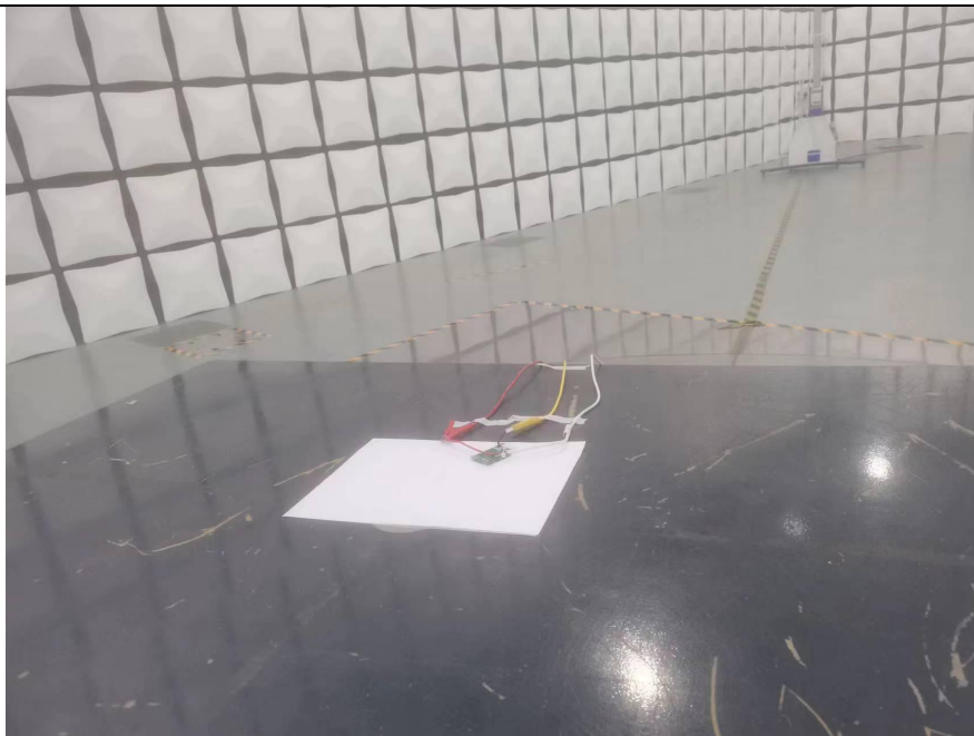
RE 30MHz~1GHz
