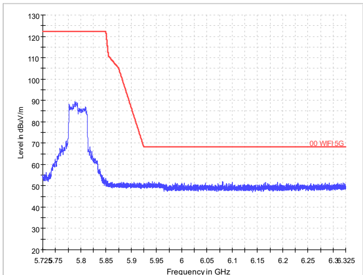
Radiated Emission Band Edge Channel No.:159 Test Mode: 802.11n Polarization: H
