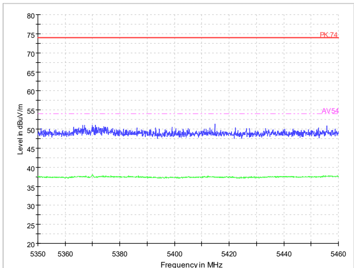
Radiated Emission Band Edge Channel No.:58 Test Mode: 802.11ac Polarization: H
