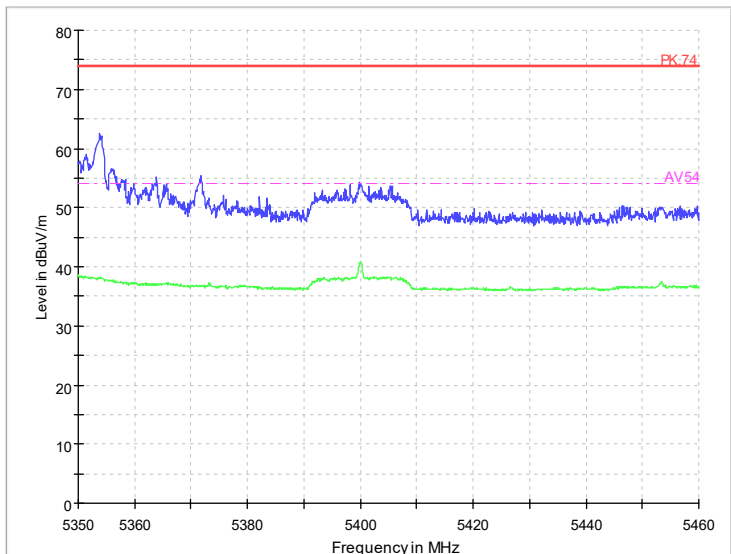
Radiated Emission Band Edge Channel No.:64 Test Mode: 802.11ac Polarization: H
