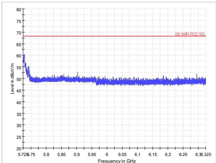
Radiated Emission Band Edge Channel No.:138 Test Mode: 802.11ac Polarization: H
