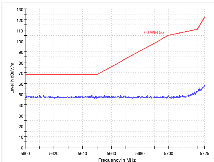
Radiated Emission Band Edge Channel No.:149 Test Mode: 802.11a Polarization: H
