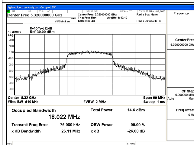
Mode:802.11ac VHT20 Frequency:5320MHz Ant:Chain0
