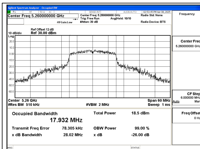
Mode:802.11ac VHT20 Frequency:5260MHz Ant:Chain0
