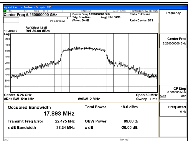
Mode:802.11ac VHT20 Frequency:5260MHz Ant:Chain1
