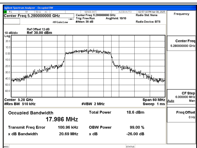
Mode:802.11ac VHT20 Frequency:5280MHz Ant:Chain0
