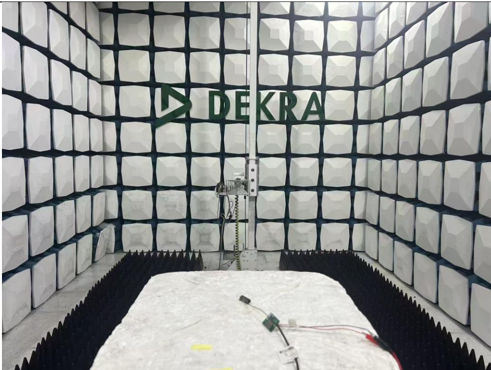
Test Location A: Radiated emission 1-18GHz
