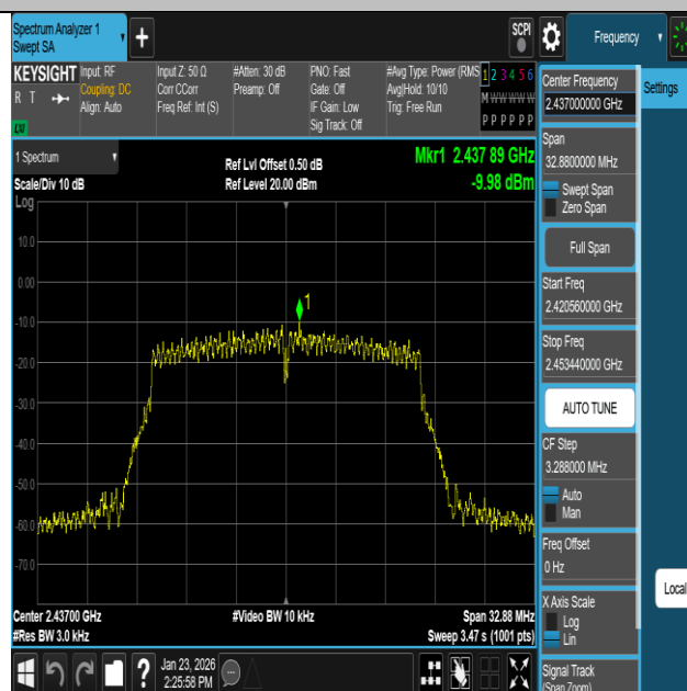
11N20SISO-Ant1-2437-PASS
