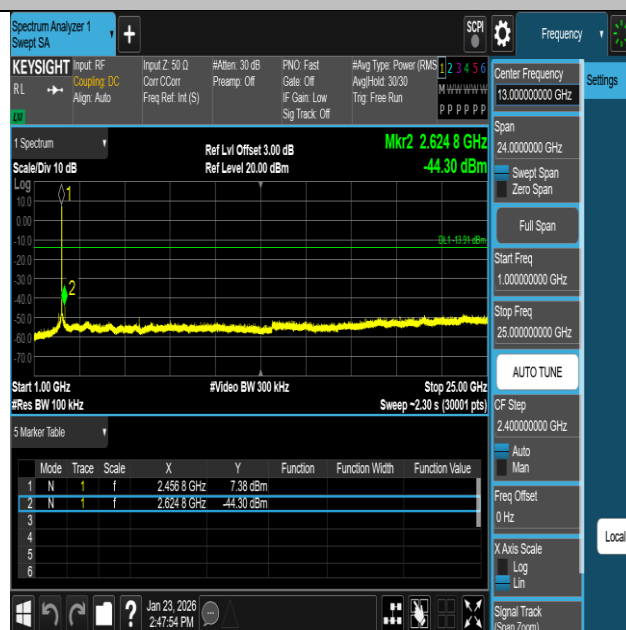
11G-Ant1-2462-1000~25000-PASS
