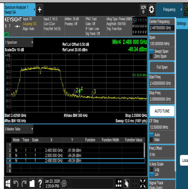
11N40SISO-Ant1-2452-PASS
