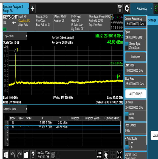
11N40SISO-Ant1-2437-1000~25000-PASS
