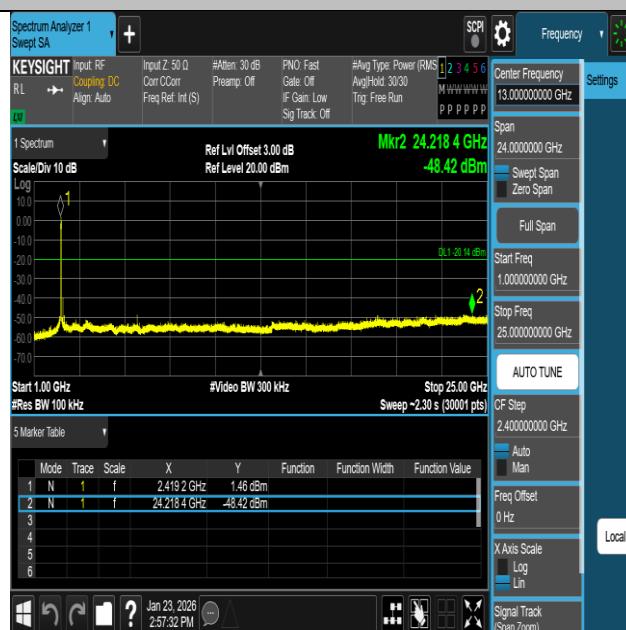
11N40SISO-Ant1-2422-1000~25000-PASS
