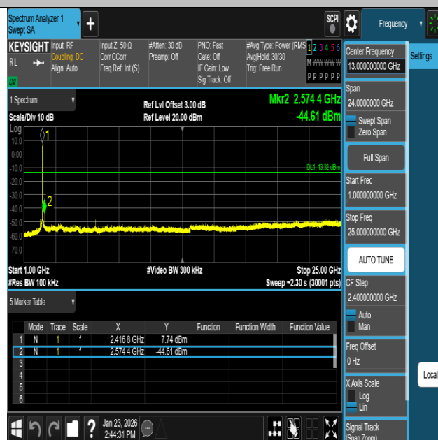
11G-Ant1-2412-1000~25000-PASS
