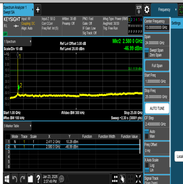
11B-Ant1-2412-1000~25000-PASS
