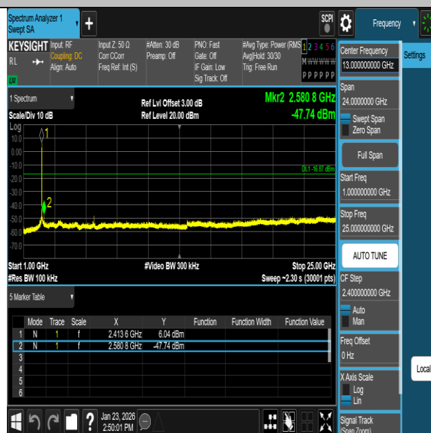
11N20SISO-Ant1-2412-1000~25000-PASS
