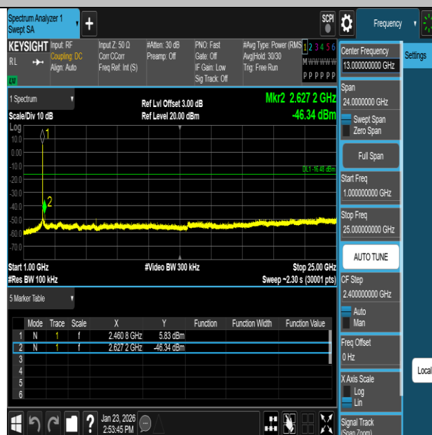
11N20SISO-Ant1-2462-1000~25000-PASS
