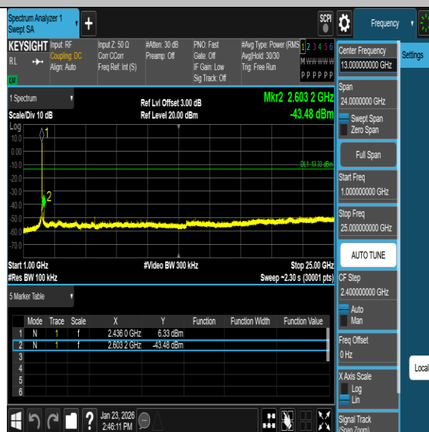
11G-Ant1-2437-1000~25000-PASS
