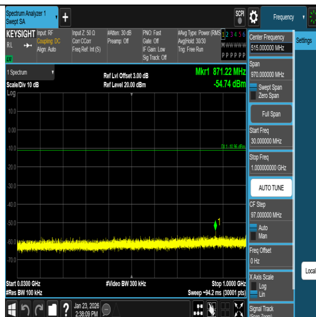
11B-Ant1-2437-30~1000-PASS
