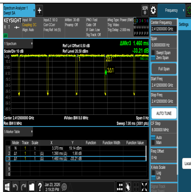
NTNV-11G-Ant1-2412
