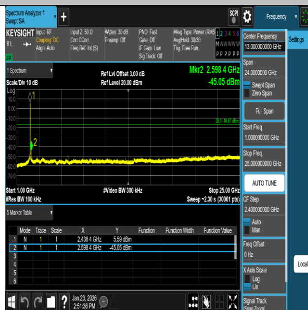
11N20SISO-Ant1-2437-1000~25000-PASS
