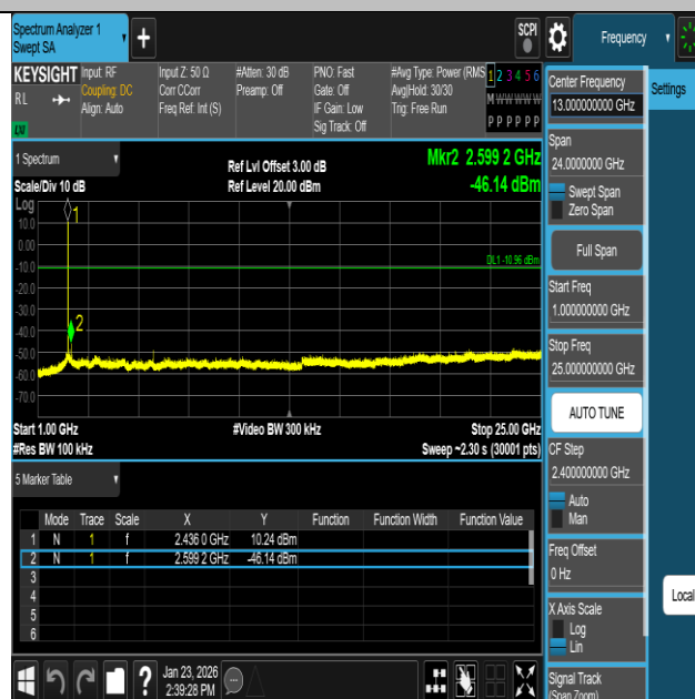
11B-Ant1-2437-1000~25000-PASS
