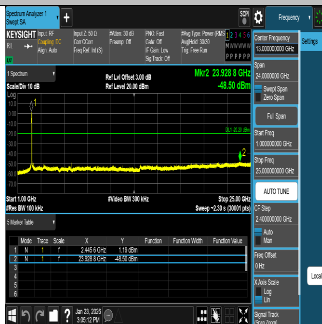
11N40SISO-Ant1-2452-1000~25000-PASS
