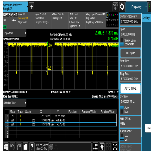
NTNV-11N20SISO-Ant1-5700
