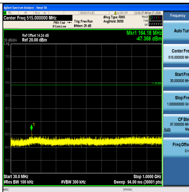
11B-Ant1-2462-30~1000-PASS
