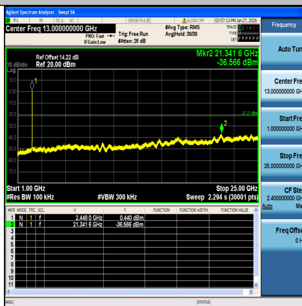
11N40SISO-Ant1-2452-1000~25000-PASS
