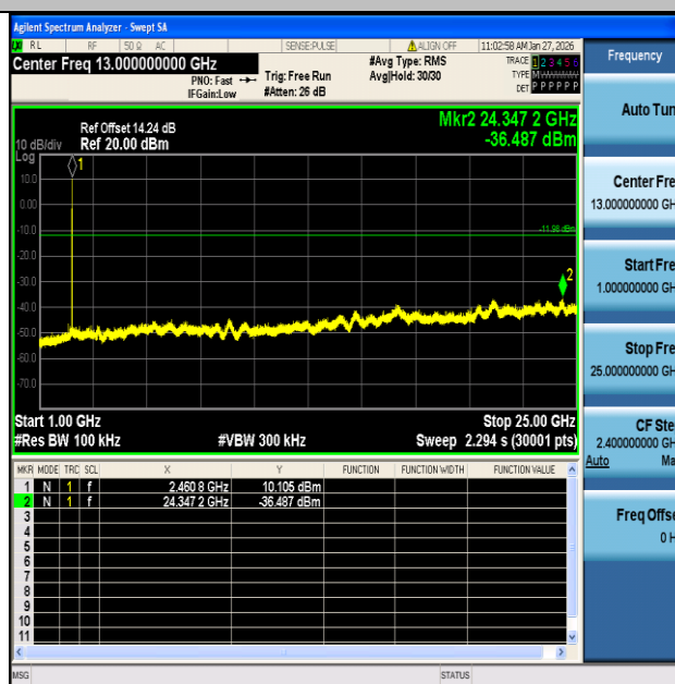
11B-Ant1-2462-1000~25000-PASS
