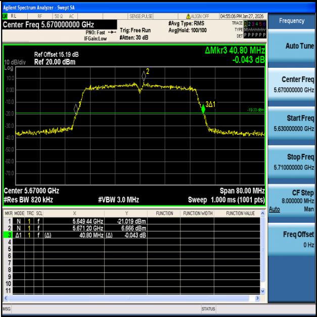
11AC40SISO-Ant1-5670
