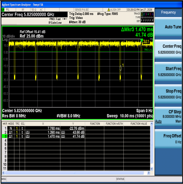
NTNV-11A-Ant1-5825
