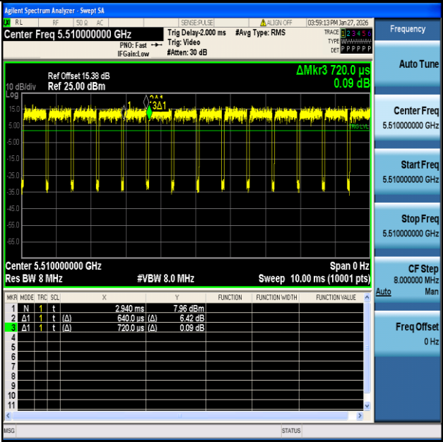
NTVN-11N40SISO-Ant1-5510
