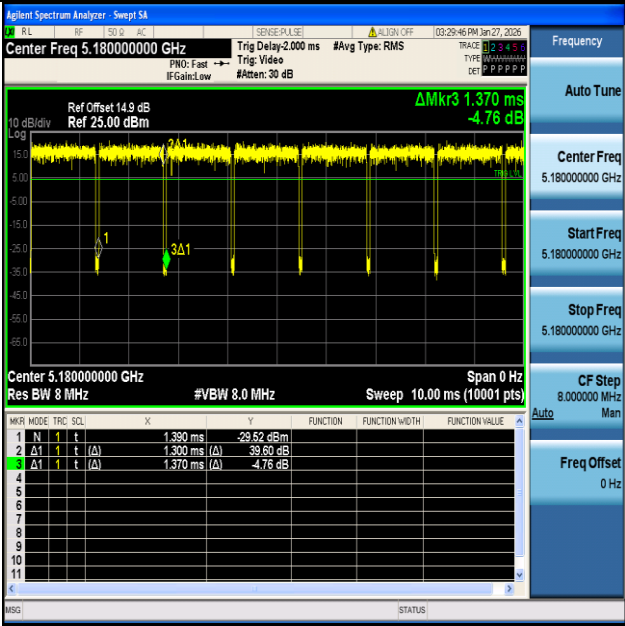
NTVN-11N20SISO-Ant1-5180
