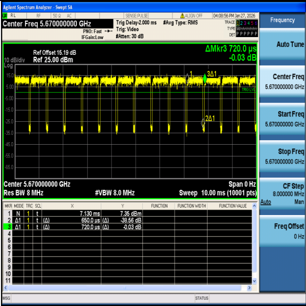
NTVN-11N40SISO-Ant1-5670
