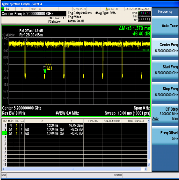
NTVN-11N20SISO-Ant1-5200
