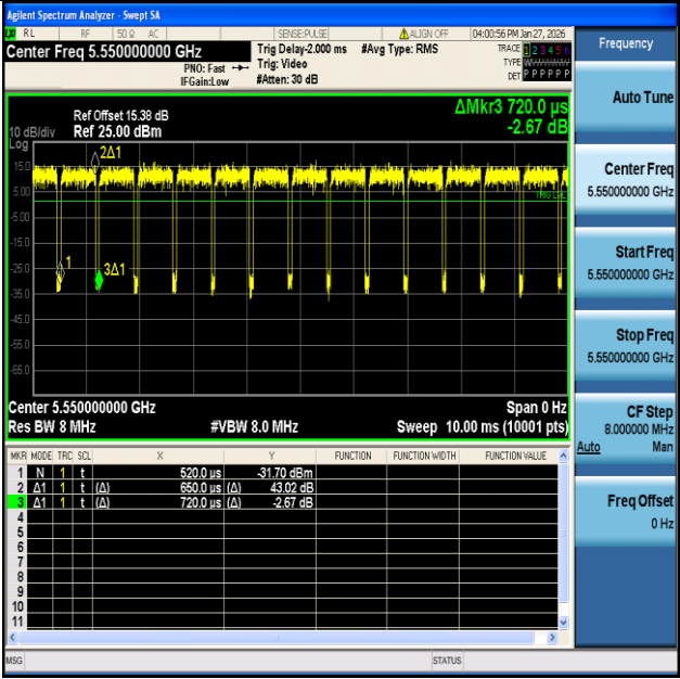
NTVN-11N40SISO-Ant1-5550
