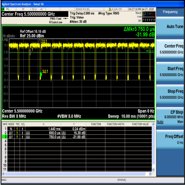
NTNV-11AC20SISO-Ant1-5500
