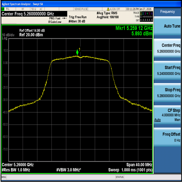
11A-Ant1-5260-PASS
