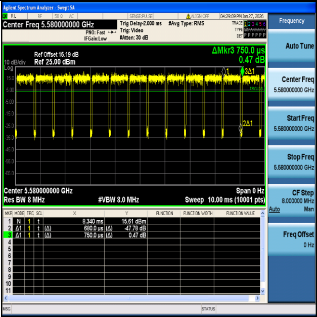
NTNV-11AC20SISO-Ant1-5580
