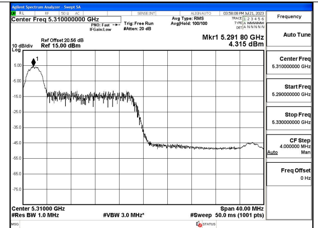
Mode:802.11ax HE40 Tone:26T Frequency:5310MHz Ant:Chain0
