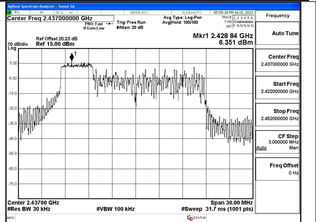
Mode:802.11ax HE20 Tone:52T Frequency:2437MHz Ant:Chain0
