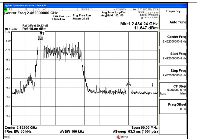
Mode:802.11ax HE40 Tone:26T Frequency:2452MHz Ant:Chain1
