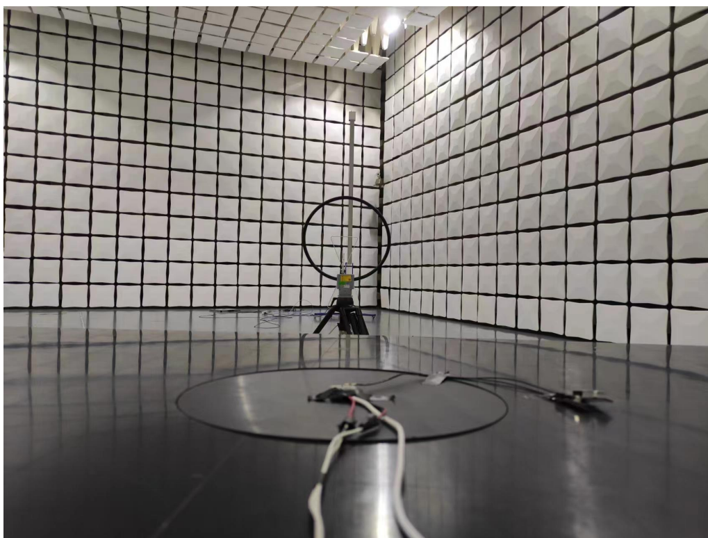
RE 9KHz~30MHz
