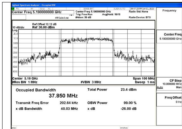
Mode:802.11ax HE40 Frequency:5190MHz Ant:Chain0
