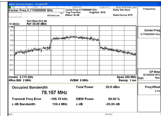
Test Mode:802.11ax HE80 5775MHz Chain1
