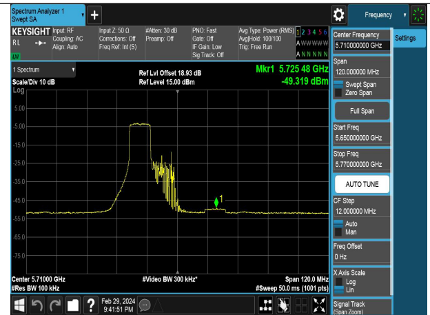
Mode:802.11ax HE40 Tone:106TR Frequency:5710MHz Ant:Chain1 scope:NII3
