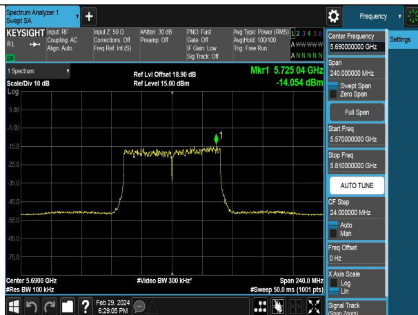
Mode:802.11ac VHT80 Frequency:5690MHz Ant:Chain0 scope:NII3
