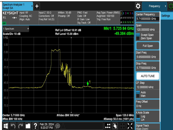
Mode:802.11ax HE40 Tone:106TR Frequency:5710MHz Ant:Chain0 scope:NII3
