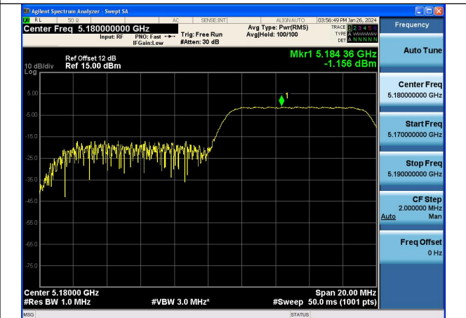
Mode:802.11ax HE20 Tone:106T Frequency:5180MHz Ant:Chain1
