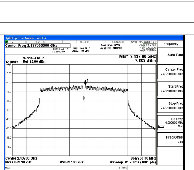
Mode:802.11n HT40 Frequency:2437MHz Ant:Chain0
