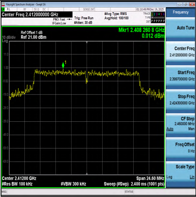
11G-2412-PASS
