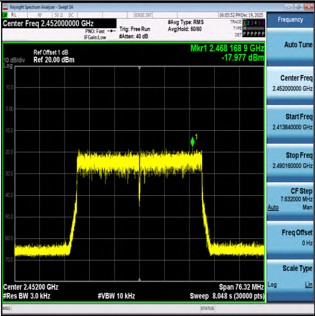
11AX40-2452-PASS
