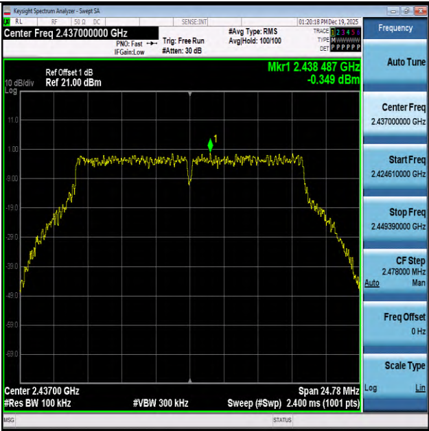
11G-2437-PASS
