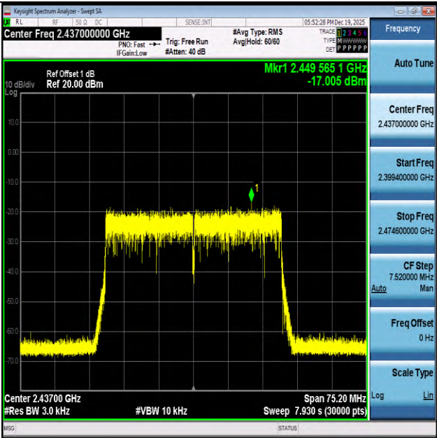
11AX40-2437-PASS
