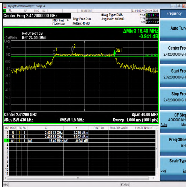
11G-2412-PASS
