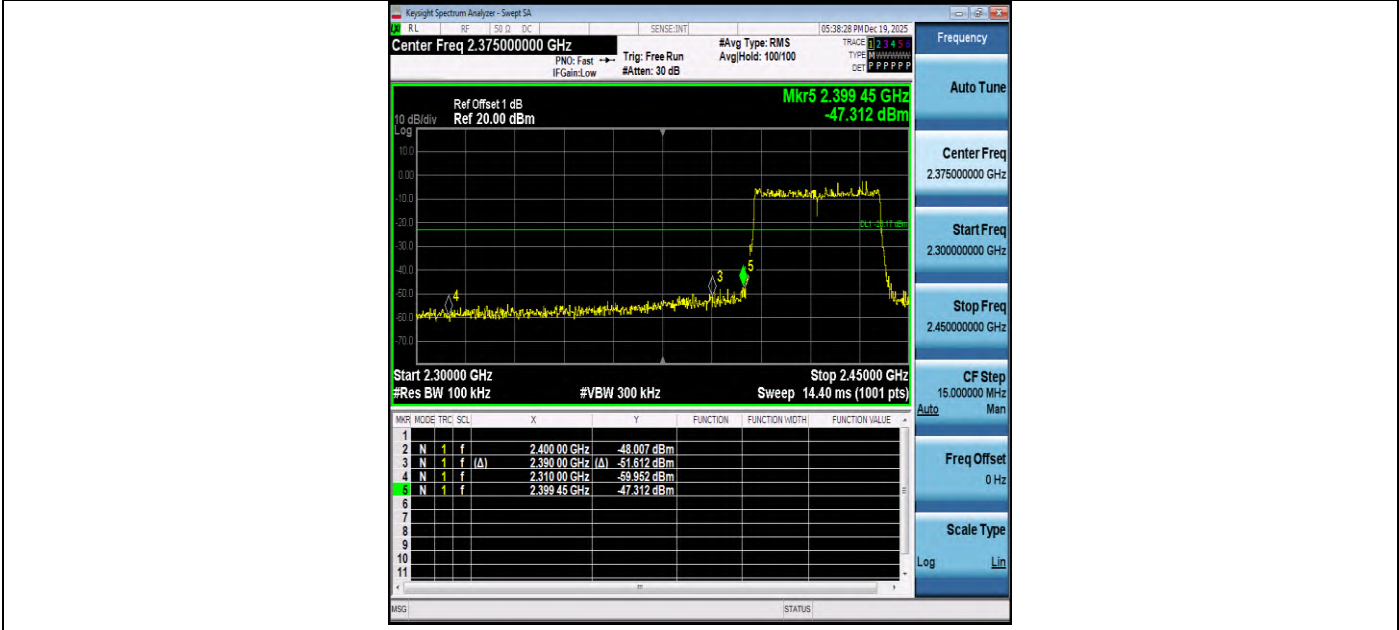
11AX40-2422-PASS
