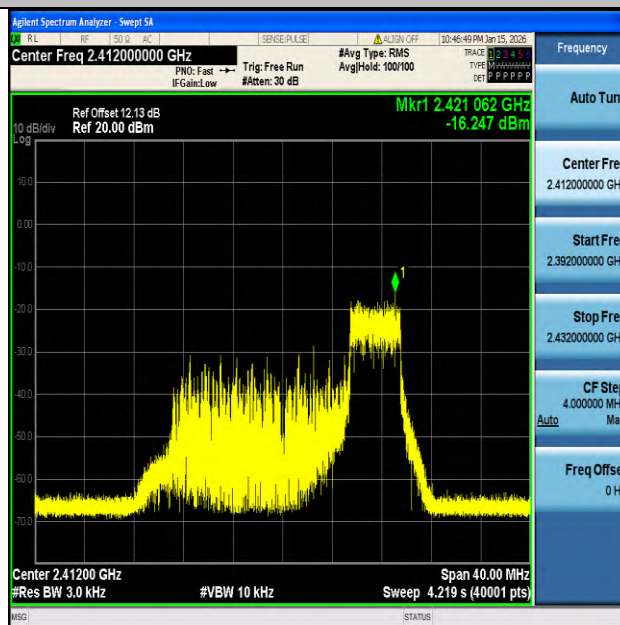
11AX20SISO-Ant1-2412-52Tone-RU37-PASS
