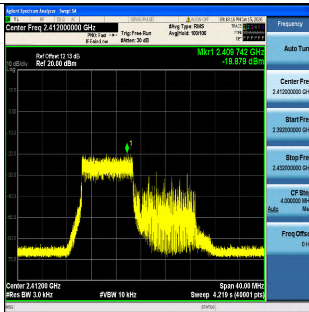
11AX20SISO-Ant1-2412-106Tone-RU53-PASS
