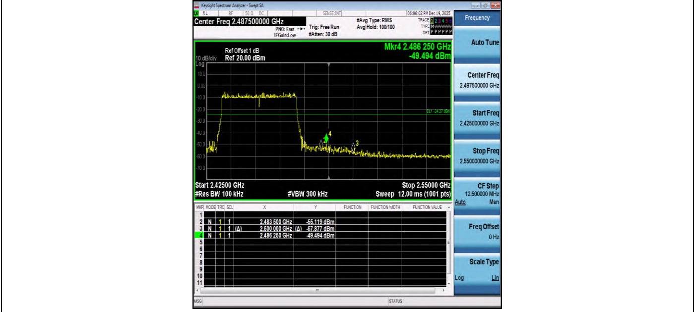
11AX40-2452-PASS
