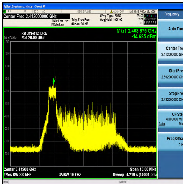
11AX20SISO-Ant1-2412-26Tone-RU0-PASS
