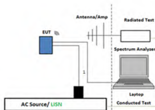
Radiate Test Below 1GHz
