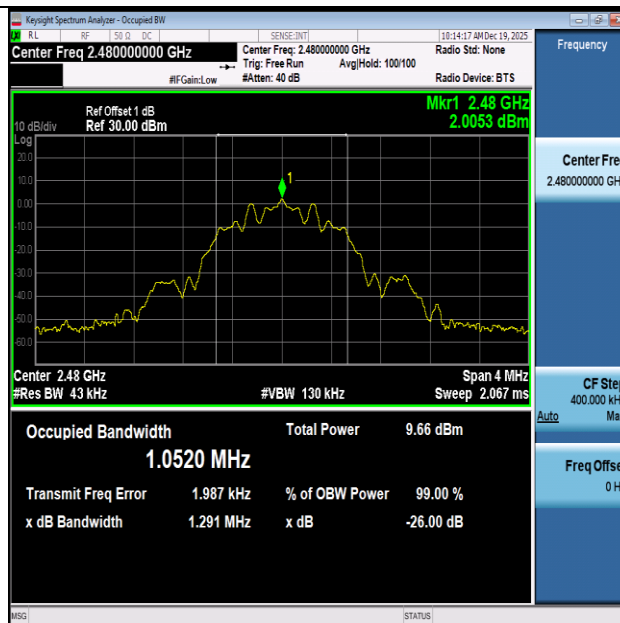
BLE_125K-2480
