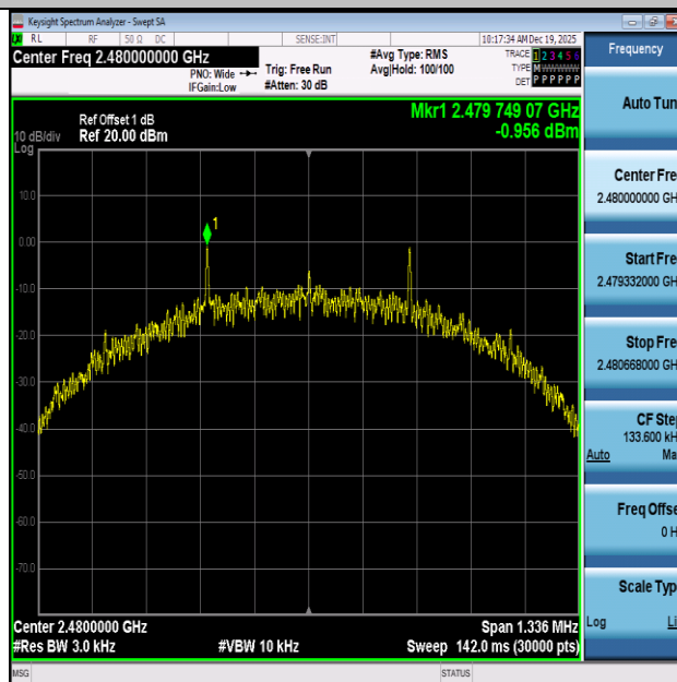
BLE_500K-2480-PASS
