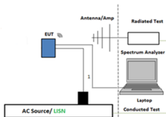
Radiate Test Below 1GHz
