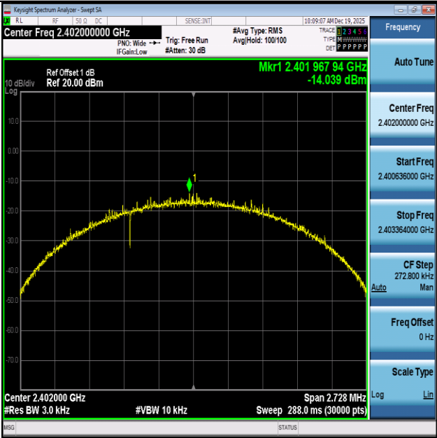
BLE_2M-2402-PASS
