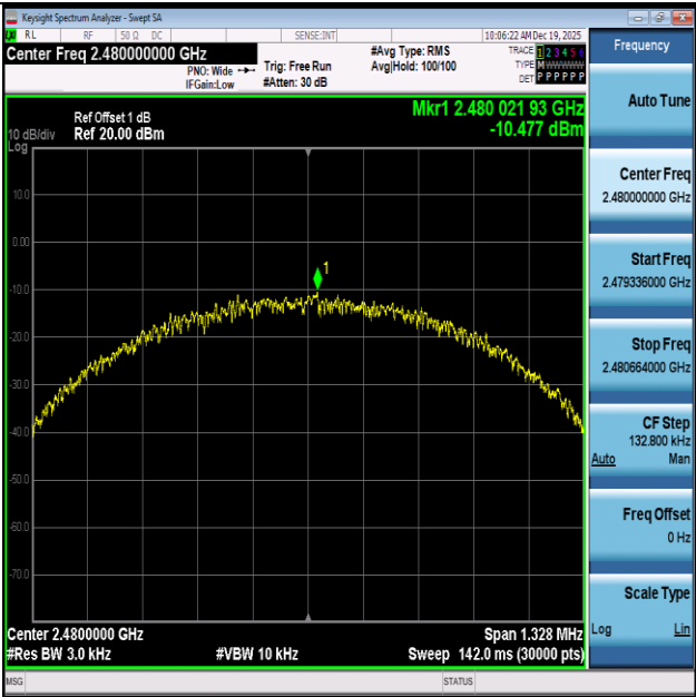
BLE_1M-2480-PASS
