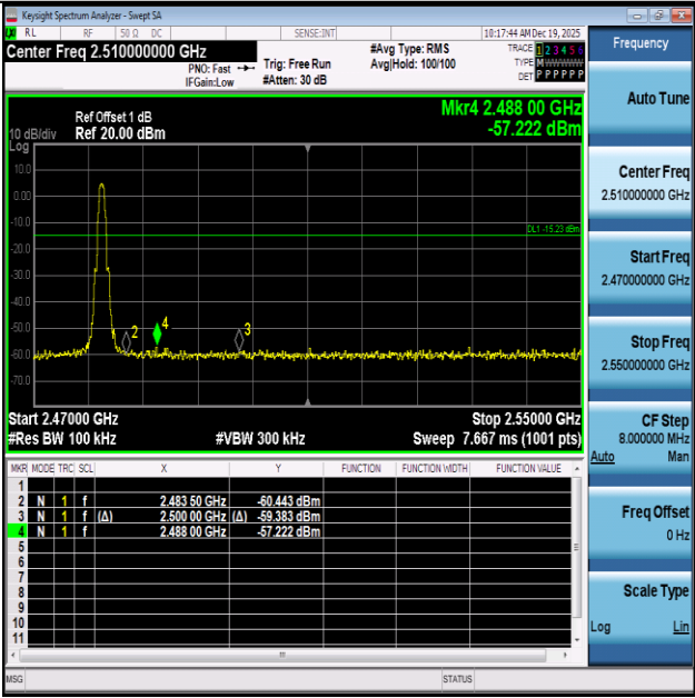
BLE_500K-2480-PASS
