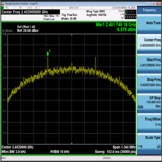
BLE_500K-2402-PASS
