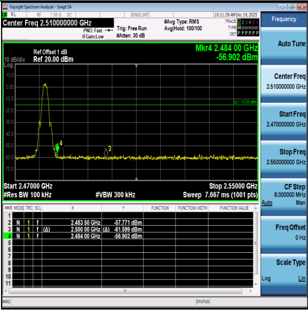
BLE_2M-2480-PASS
