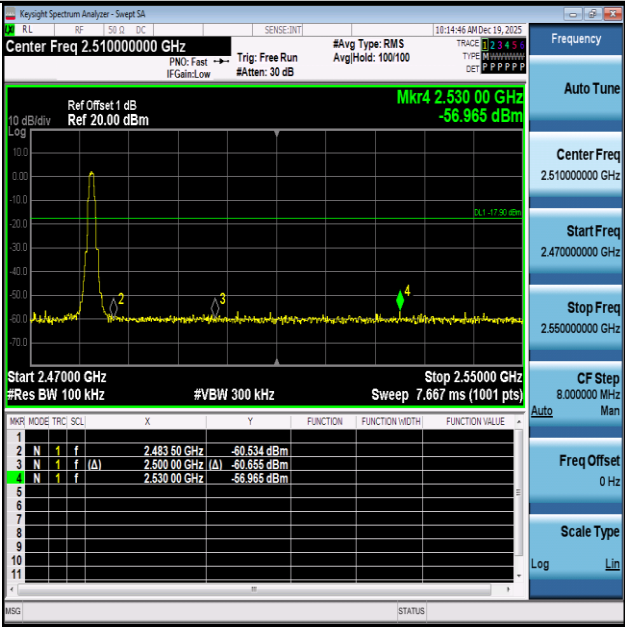
BLE_125K-2480-PASS
