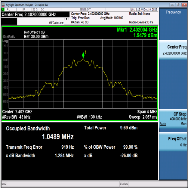
BLE_125K-2402
