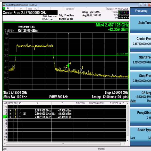
11AX40SISO-Ant1-2452-PASS
