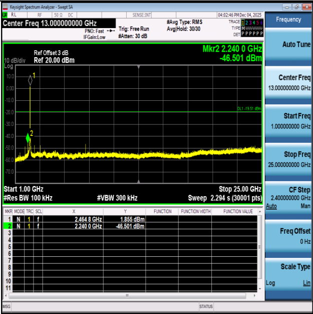
11AX40SISO-Ant1-2452-1000~25000-PASS
