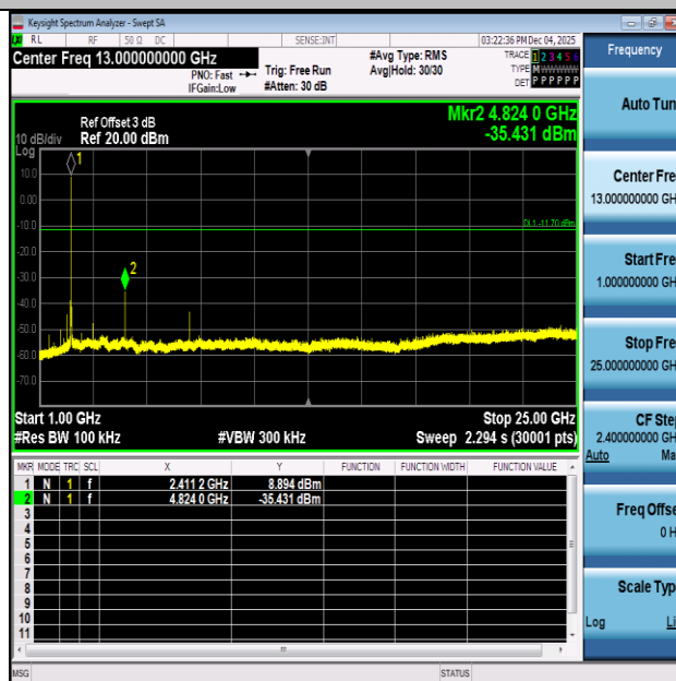
11B-Ant1-2412-1000~25000-PASS
