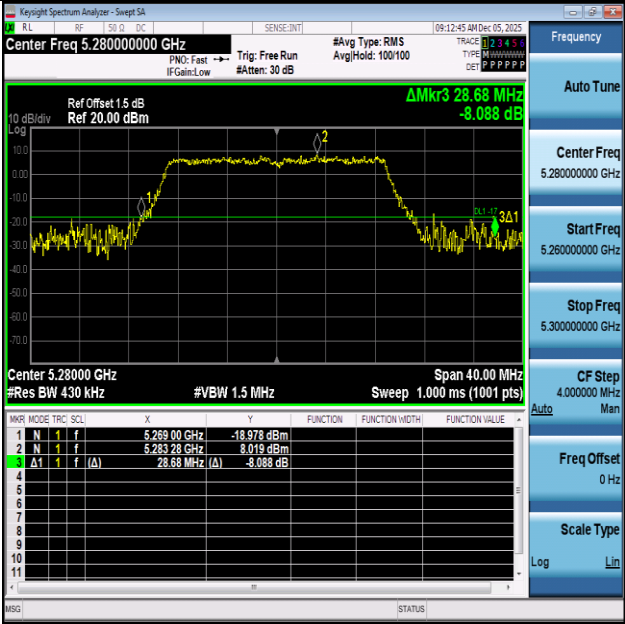
11N20SISO-Ant1-5280
