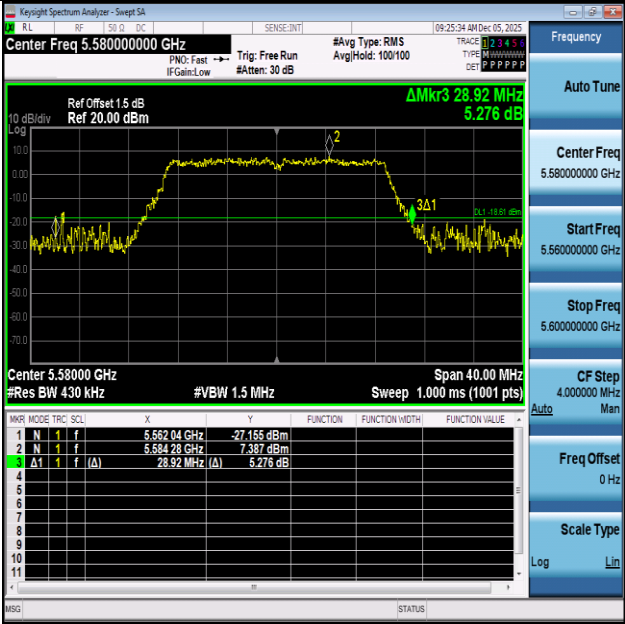
11N20SISO-Ant1-5580
