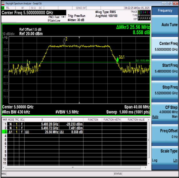
11N20SISO-Ant1-5500
