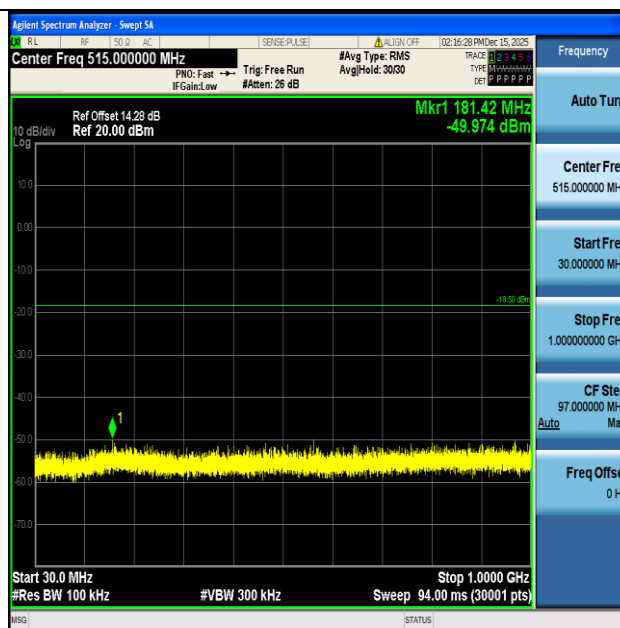
11AX20SISO-Ant1-2437-30~1000-PASS
