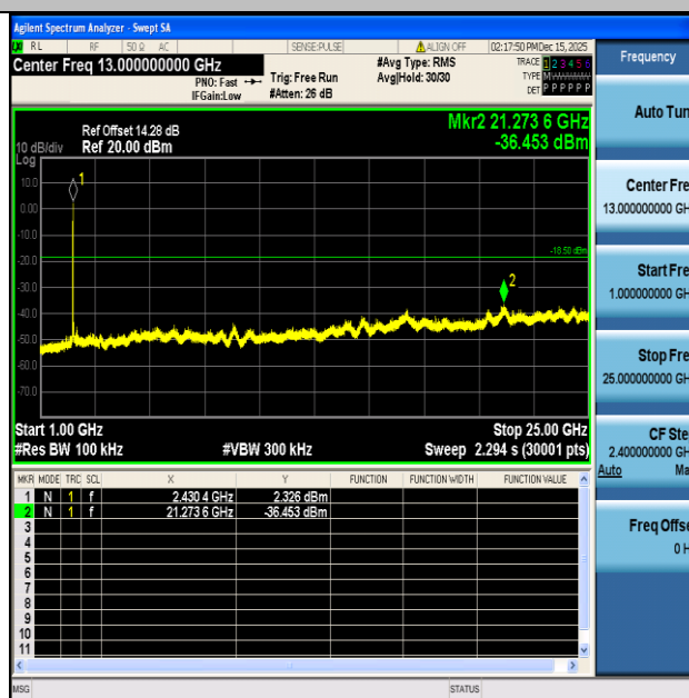
11AX20SISO-Ant1-2437-1000~25000-PASS
