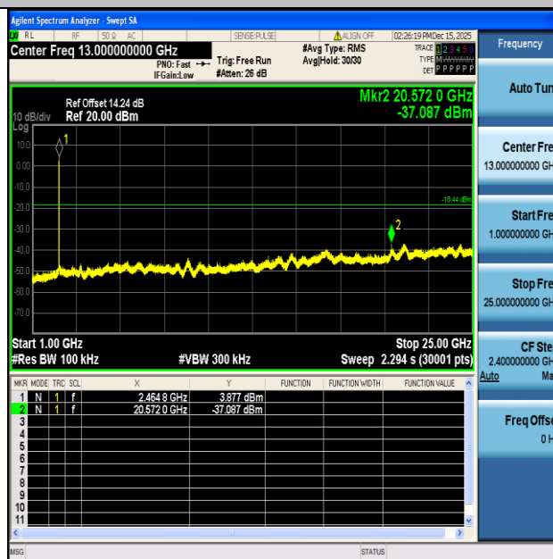
11AX20SISO-Ant1-2462-1000~25000-PASS
