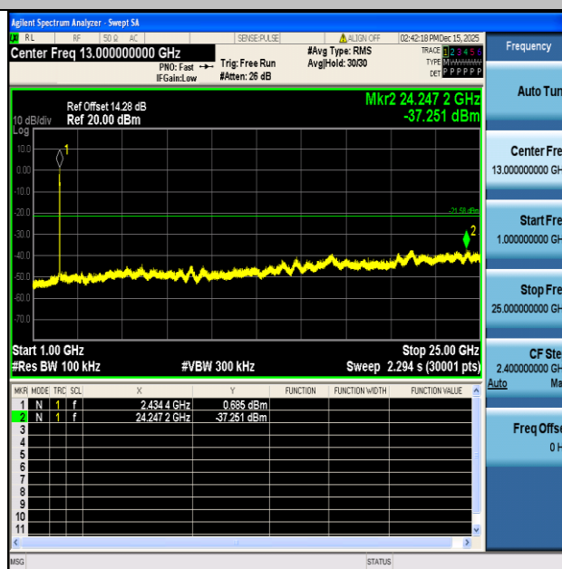
11AX40SISO-Ant1-2437-1000~25000-PASS
