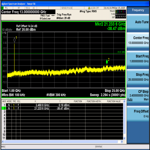
11N20SISO-Ant1-2462-1000~25000-PASS
