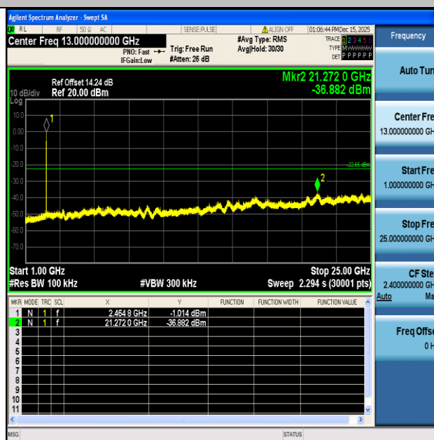
11G-Ant1-2462-1000~25000-PASS
