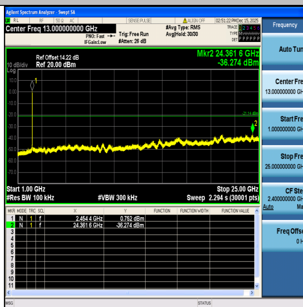
11AX40SISO-Ant1-2452-1000~25000-PASS
