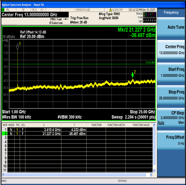
11AX20SISO-Ant1-2412-1000~25000-PASS
