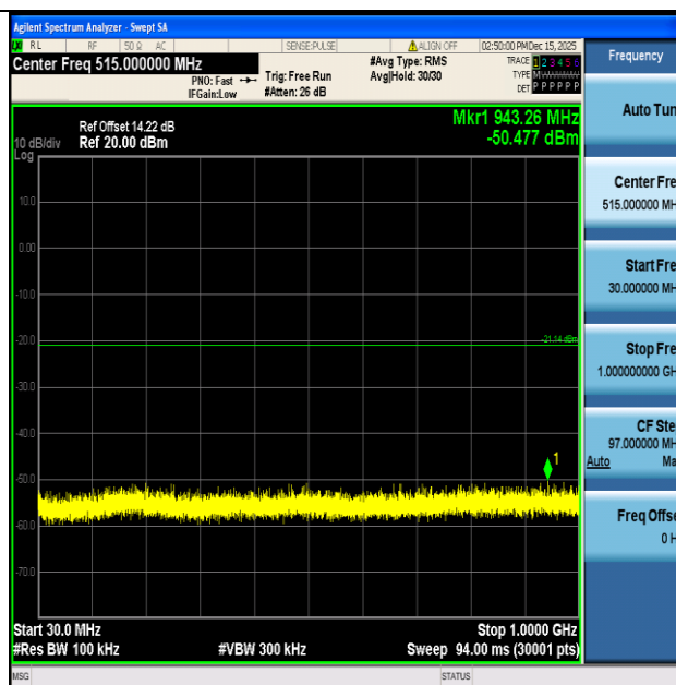
11AX40SISO-Ant1-2452-30~1000-PASS
