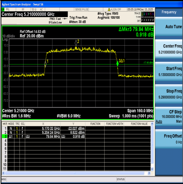
11AC80ISO-Ant1-5210
