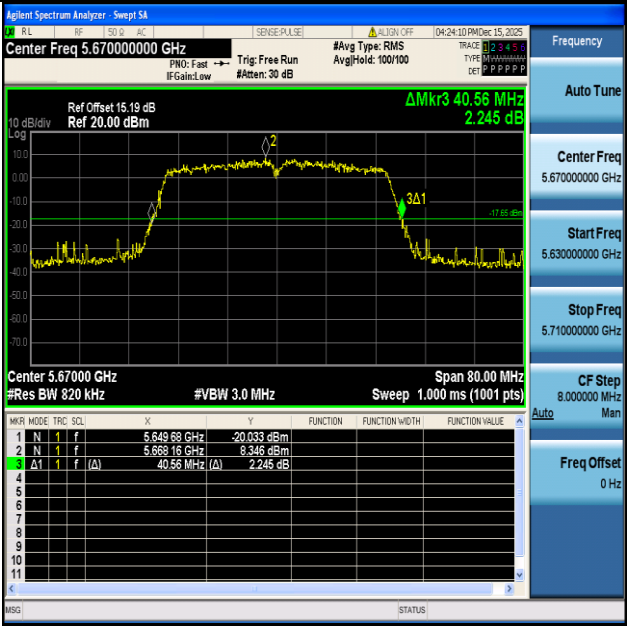
11N40SISO-Ant1-5670
