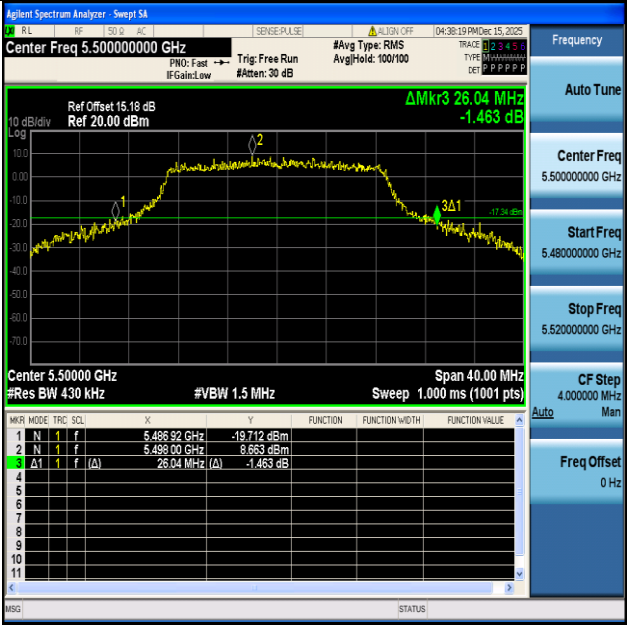
11AC20SISO-Ant1-5500
