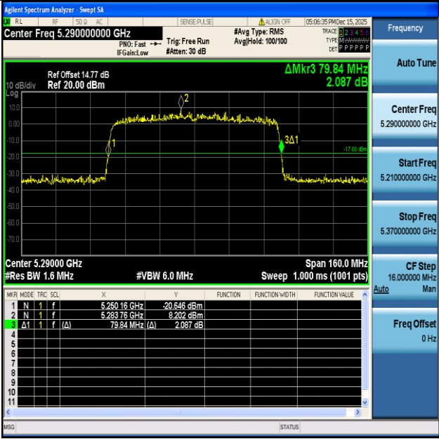
11AC80ISO-Ant1-5290
