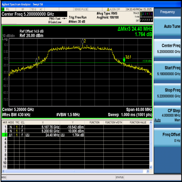
11AC20SISO-Ant1-5200
