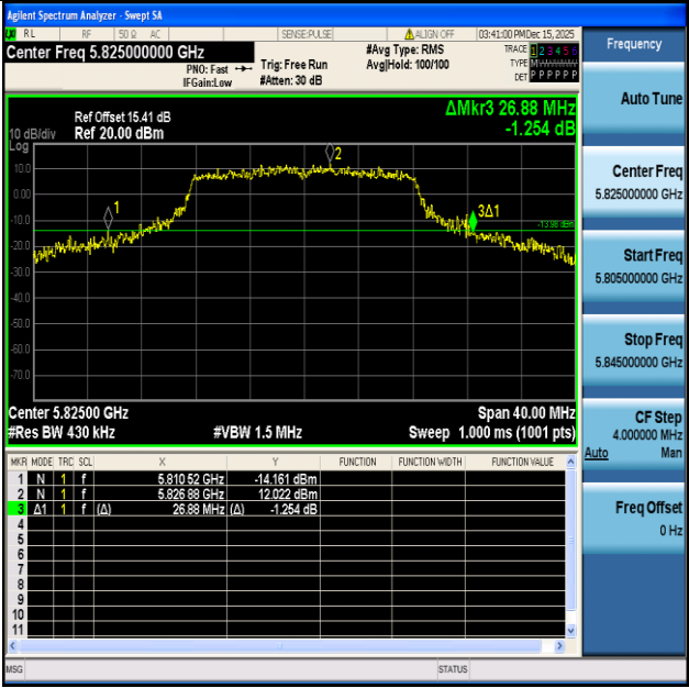
11A-Ant1-5825
