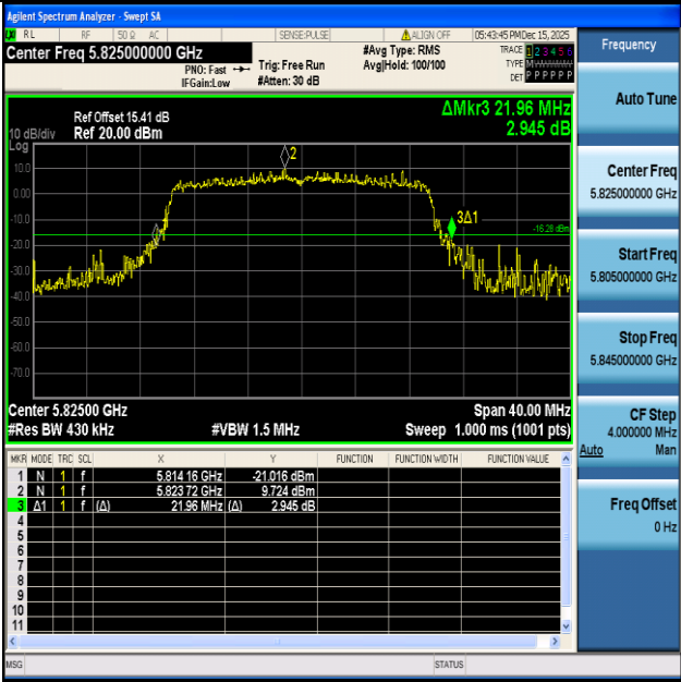
11AX20ISO-Ant1-5825
