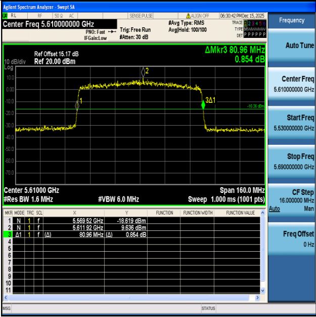
11AX80ISO-Ant1-5610
