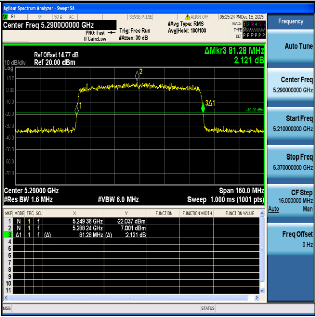
11AX80ISO-Ant1-5290
