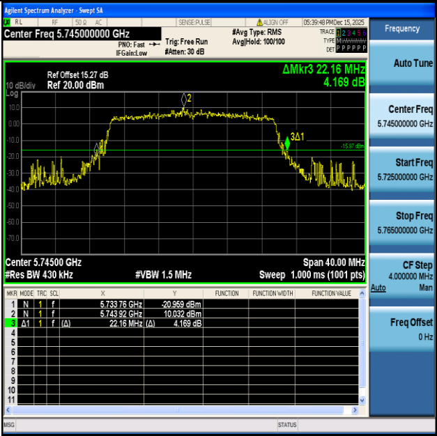
11AX20ISO-Ant1-5745
