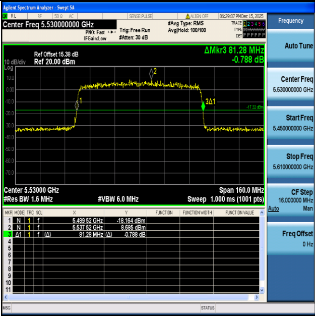
11AX80ISO-Ant1-5530
