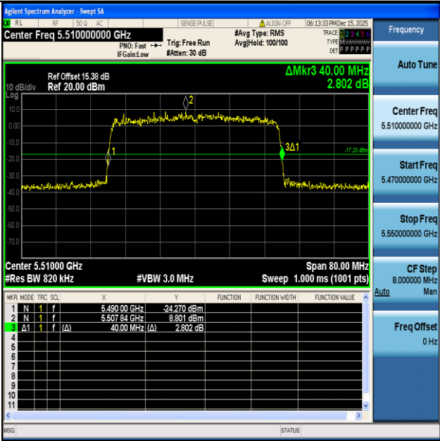
11AX40ISO-Ant1-5510
