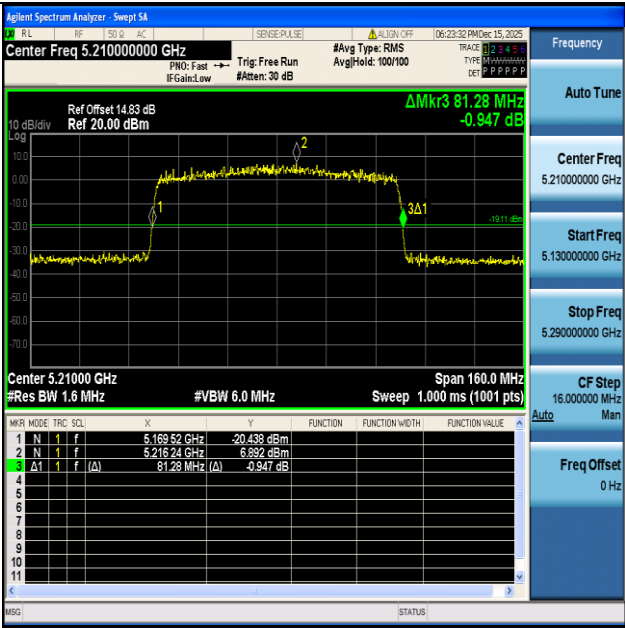
11AX80ISO-Ant1-5210
