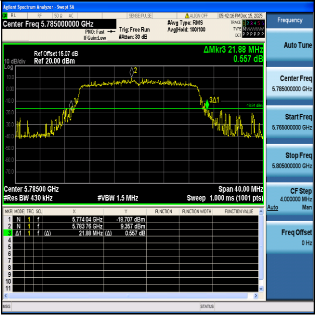
11AX20ISO-Ant1-5785
