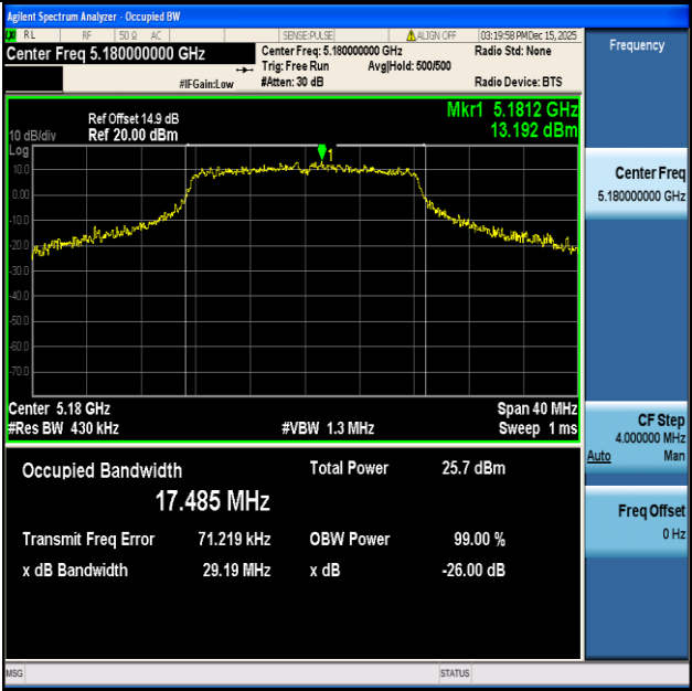
11A-Ant1-5180
