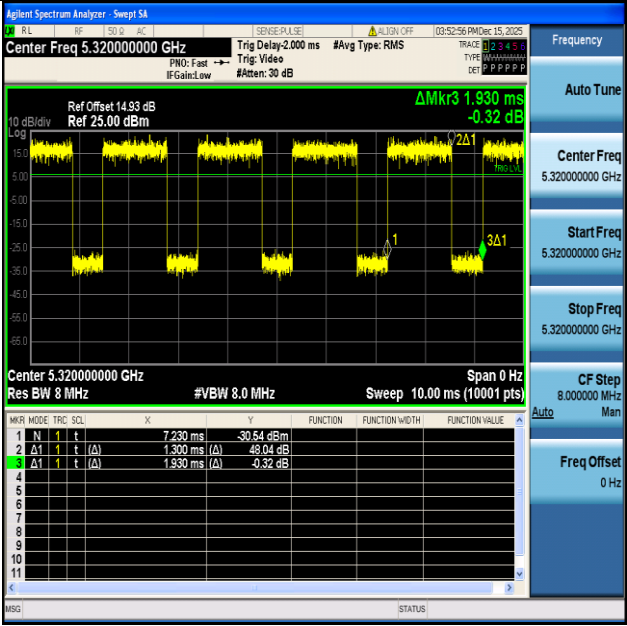
NTVN-11N20SISO-Ant1-5320
