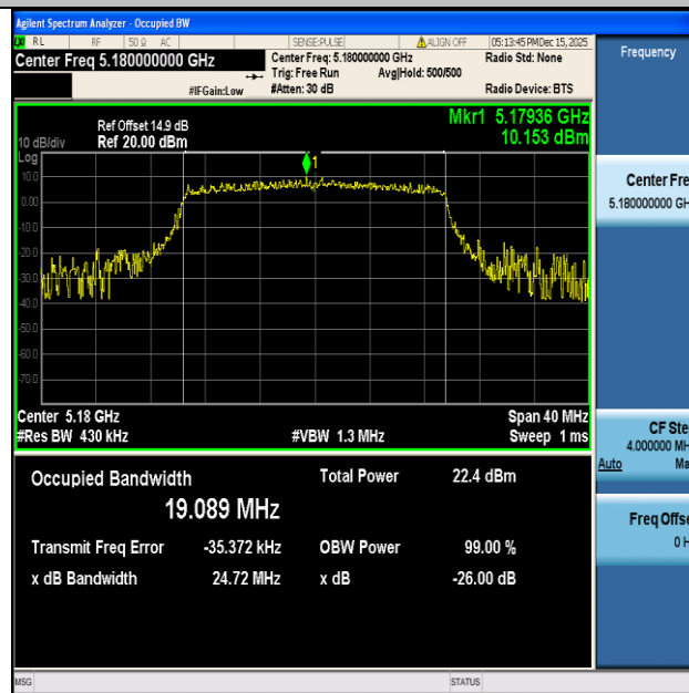
11AX20ISO-Ant1-5180
