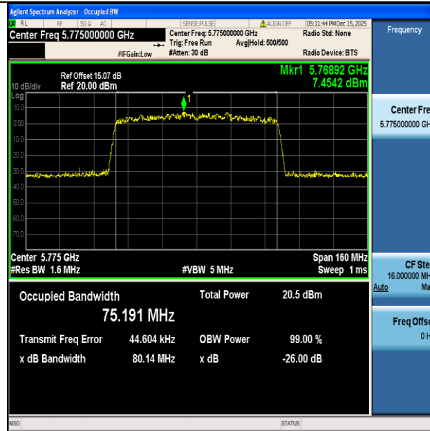
11AC80ISO-Ant1-5775
