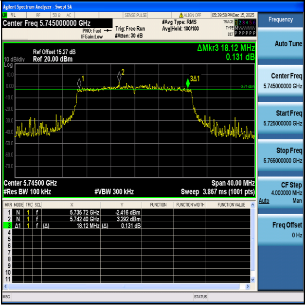
11AX20SISO-Ant1-5745-PASS
