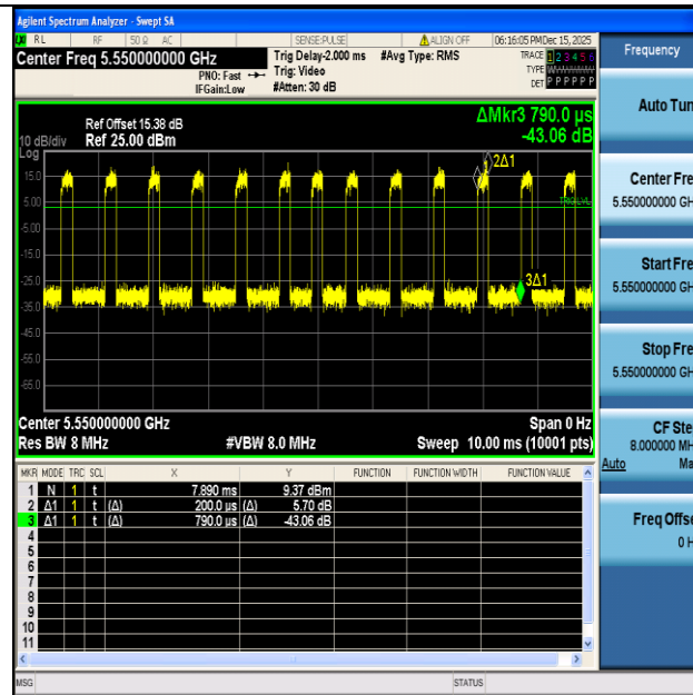
NTNV-11AX40SISO-Ant1-5550
