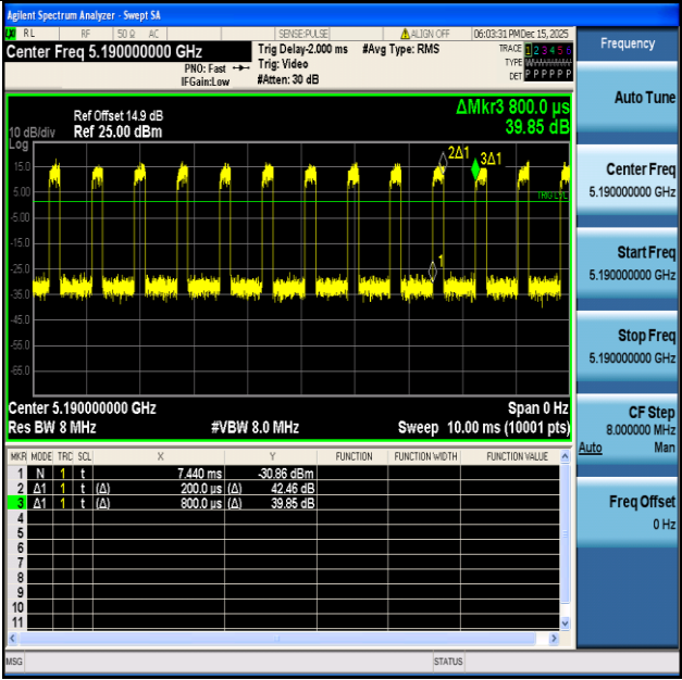
NTNV-11AX40SISO-Ant1-5190
