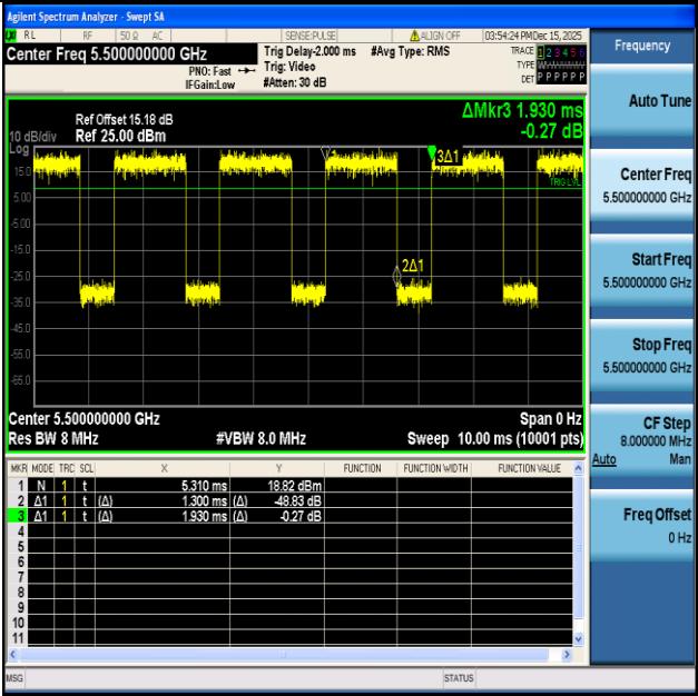
NTVN-11N20SISO-Ant1-5500
