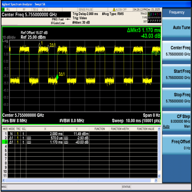
NTVN-11N40SISO-Ant1-5755
