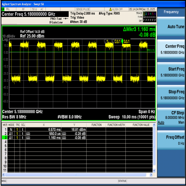
NTNV-11AX20SISO-Ant1-5180
