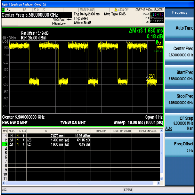
NTVN-11N20SISO-Ant1-5580
