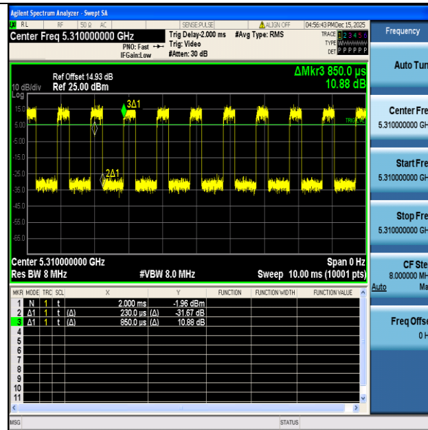
NTNV-11AC40SISO-Ant1-5310
