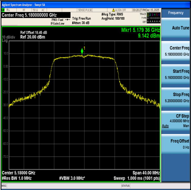
11A-Ant1-5180-PASS
