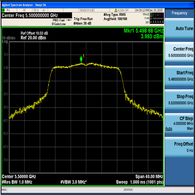
11AC20SISO-Ant1-5500-PASS
