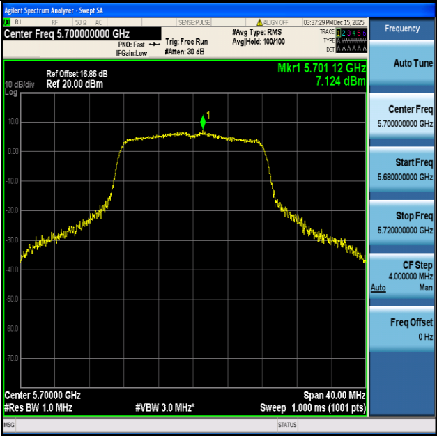
11A-Ant1-5700-PASS
