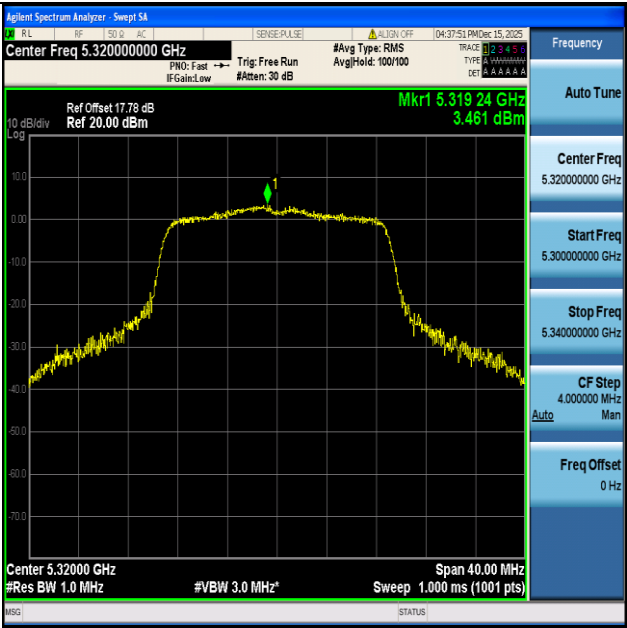
11AC20SISO-Ant1-5320-PASS
