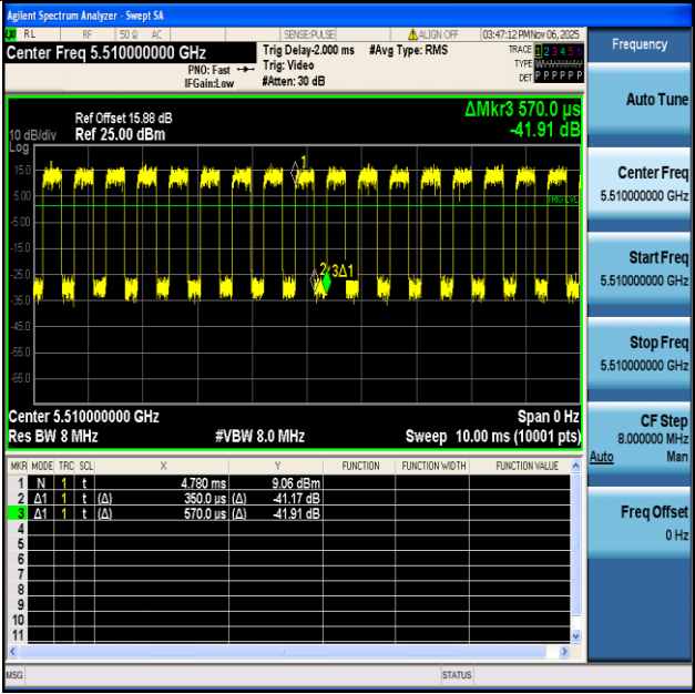
NTNV-11AC40SISO-Ant1-5550
