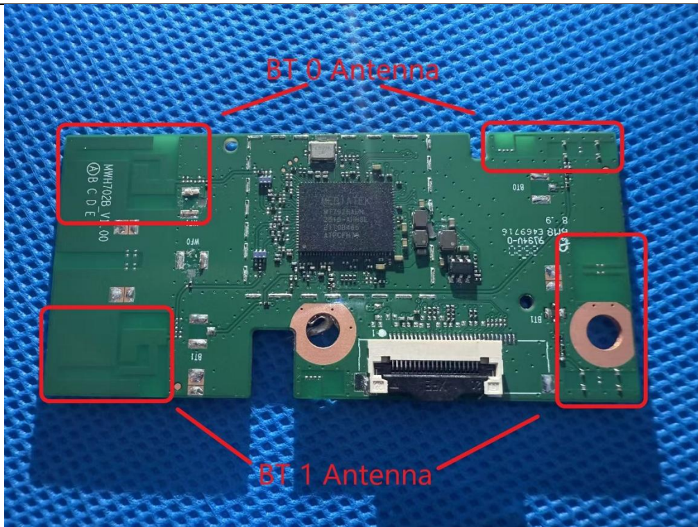
EUT Photo(5) BT Antenna
