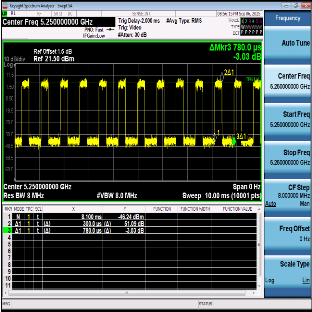
NTNV-11AX160SISO-Ant1-5250
