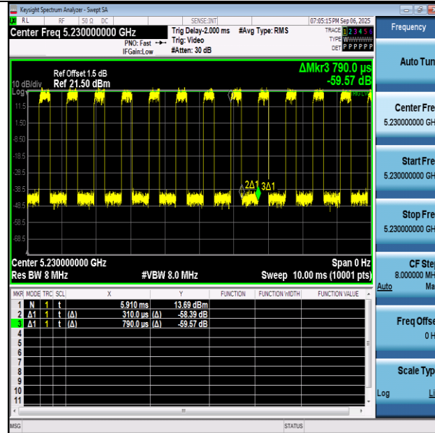
NTNV-11AX40SISO-Ant1-5230
