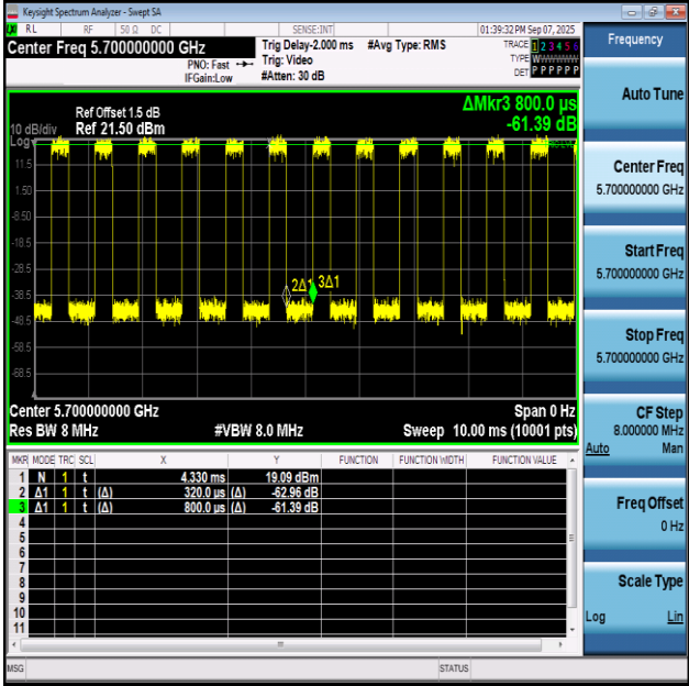
NTNV-11BE20SISO-Ant1-5700
