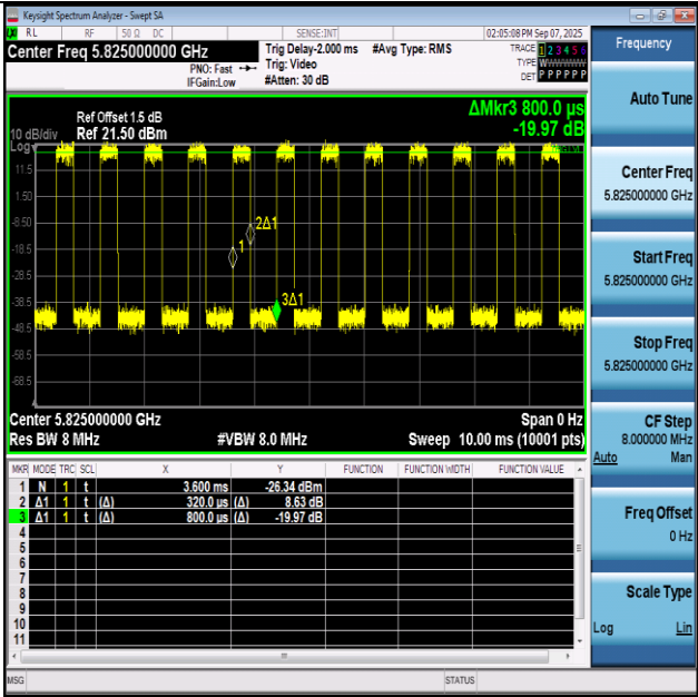
NTNV-11BE20SISO-Ant1-5825
