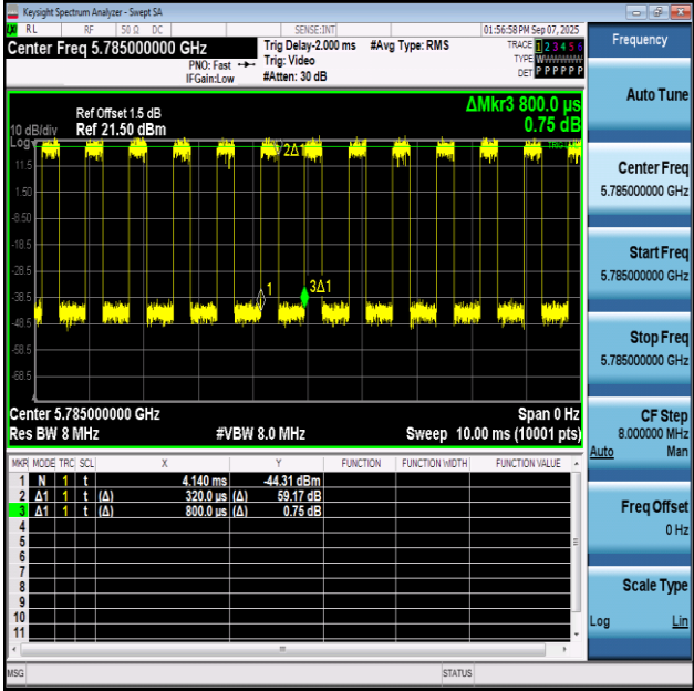
NTNV-11BE20SISO-Ant1-5785
