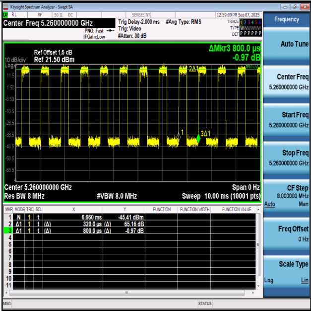
NTNV-11BE20SISO-Ant1-5260
