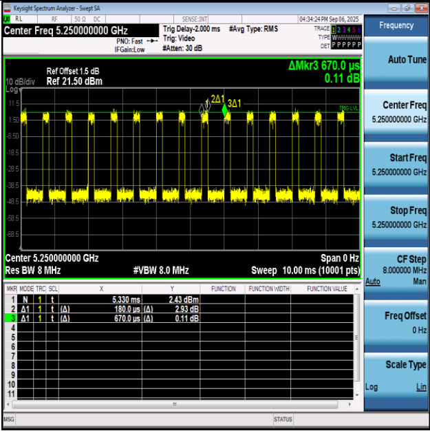
NTNV-11AC160SISO-Ant1-5250
