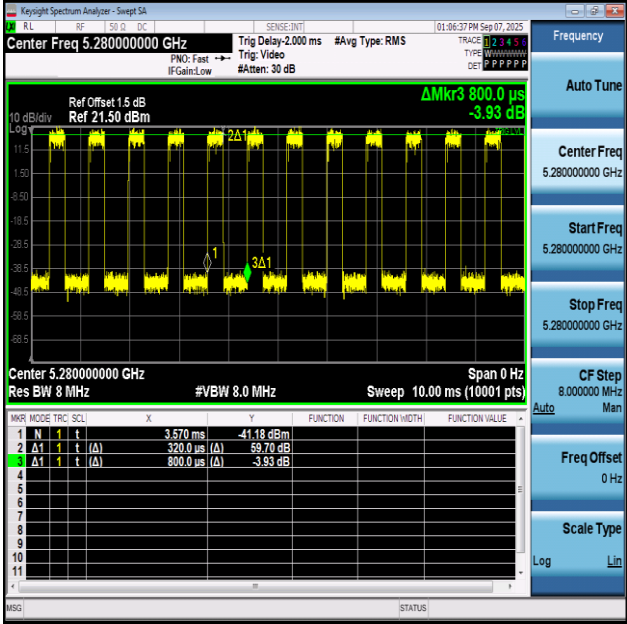
NTNV-11BE20SISO-Ant1-5280
