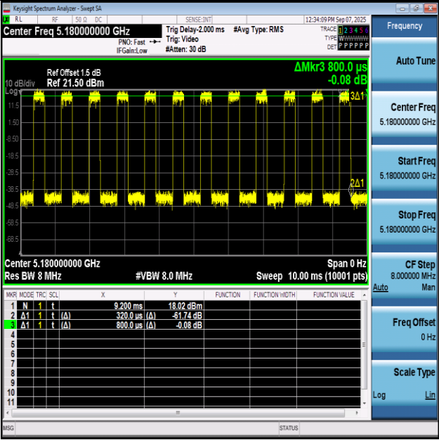
NTNV-11BE20SISO-Ant1-5180
