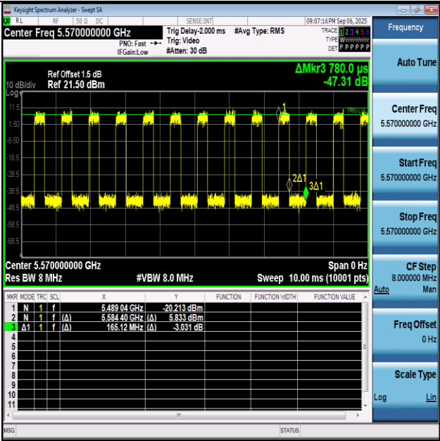
NTNV-11AX160SISO-Ant1-5570
