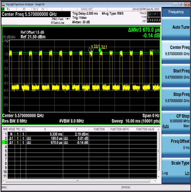
NTNV-11AC160SISO-Ant1-5570
