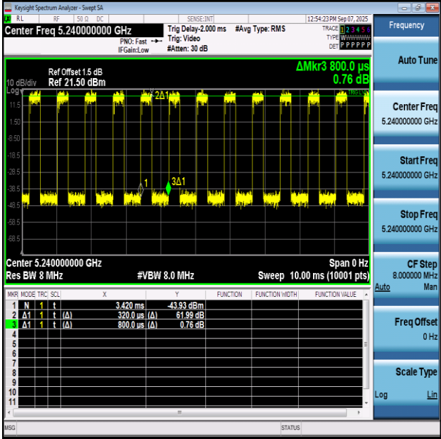
NTNV-11BE20SISO-Ant1-5240
