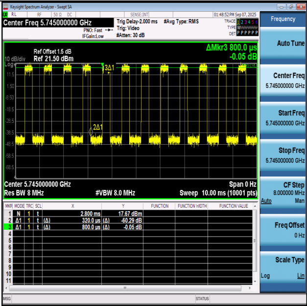
NTNV-11BE20SISO-Ant1-5745
