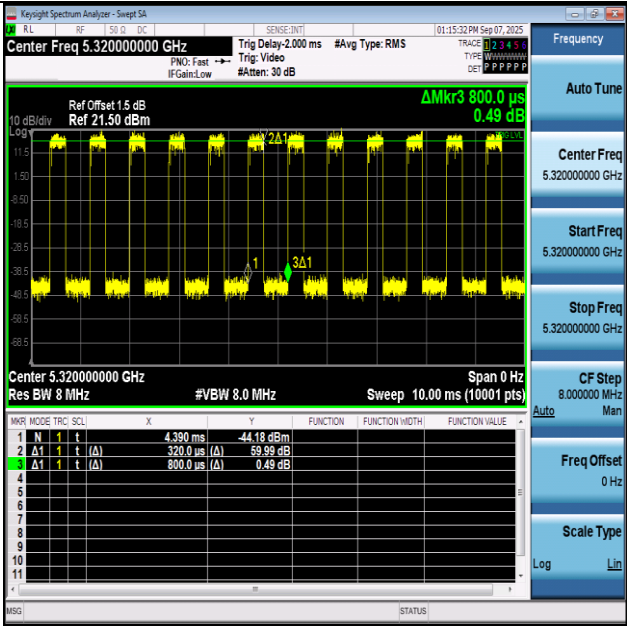
NTNV-11BE20SISO-Ant1-5320
