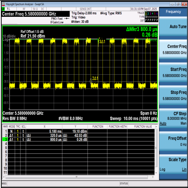
NTNV-11BE20SISO-Ant1-5580
