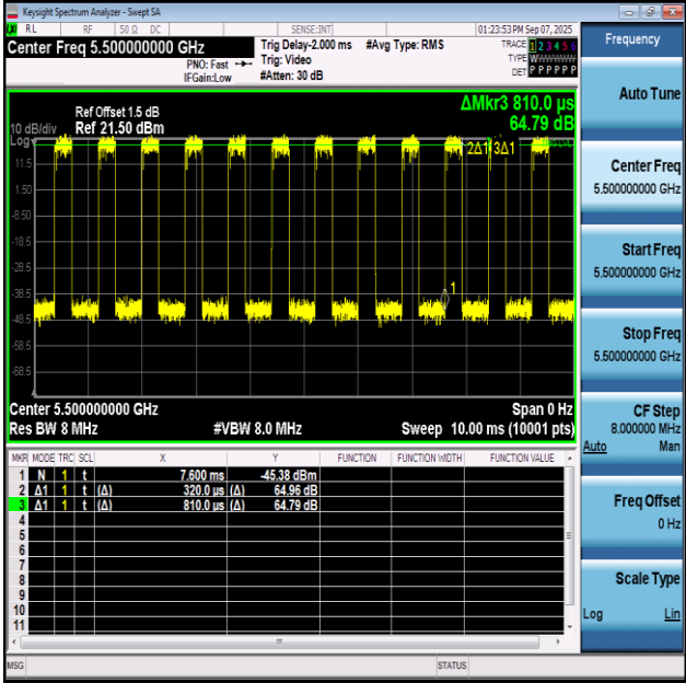
NTNV-11BE20SISO-Ant1-5500
