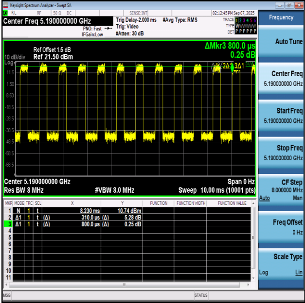
NTNV-11BE40SISO-Ant1-5190
