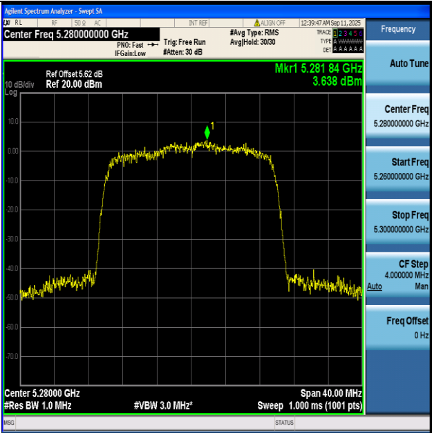
11AX20-Ant1+2-5280-PASS
