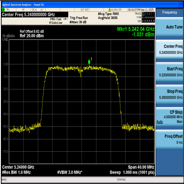
11AX20-Ant1+2-5240-PASS
