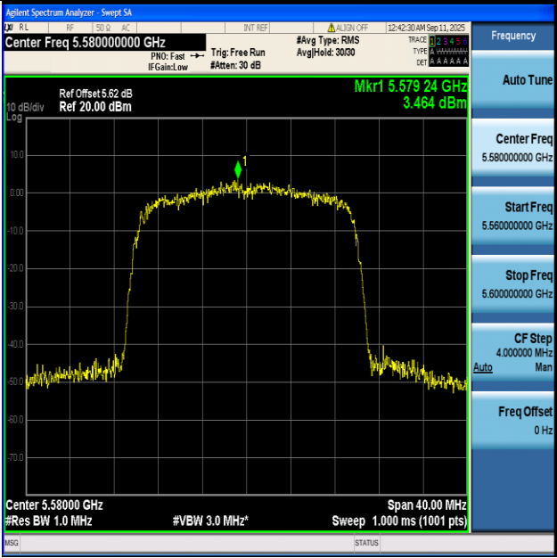
11AX20-Ant1+2-5580-PASS
