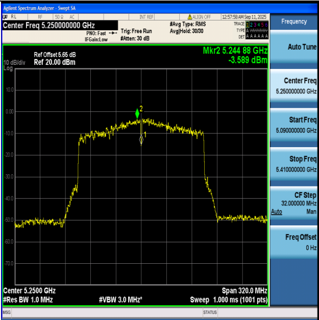
11AX160-Ant1+2-5250_UNII-1-PASS
