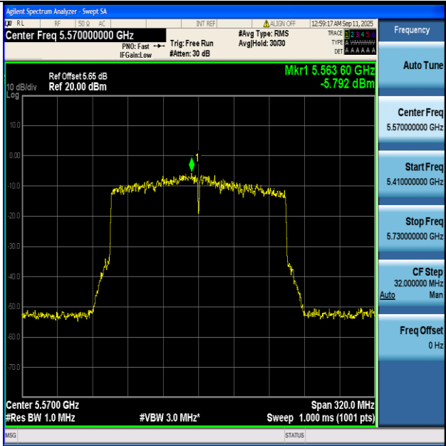
11AX160-Ant1+2-5570-PASS
