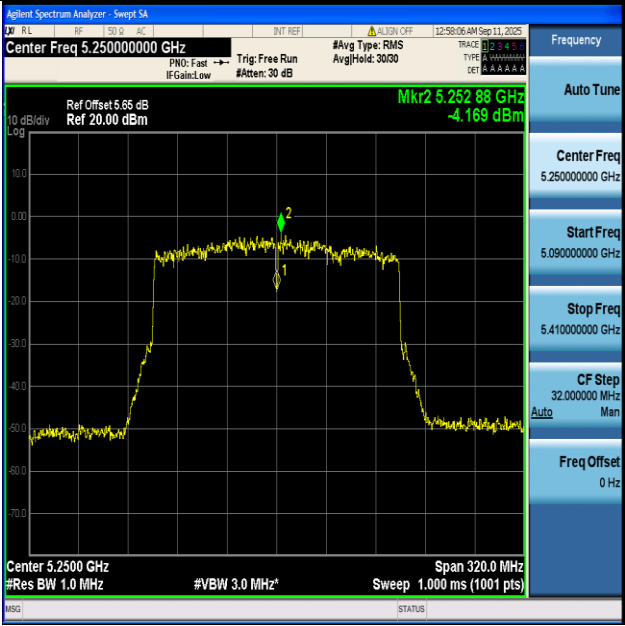
11AX160-Ant1+2-5250_UNII-2A-PASS
