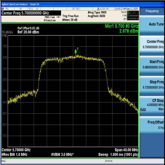
11AX20-Ant1+2-5700-PASS
