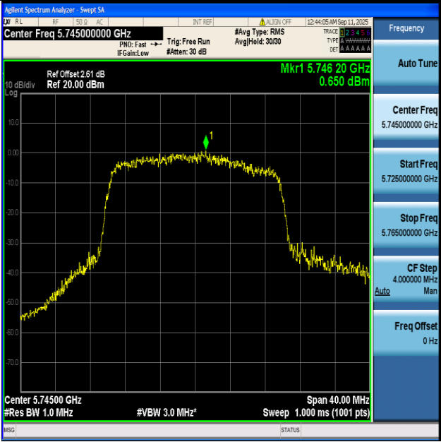
11AX20-Ant1+2-5745-PASS
