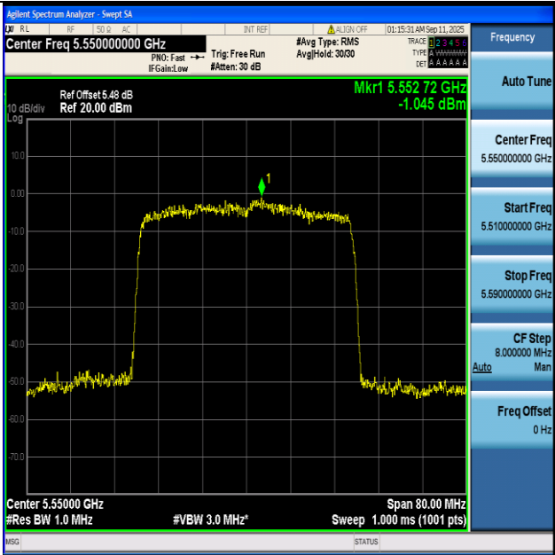
11BE40-Ant1+2-5550-PASS
