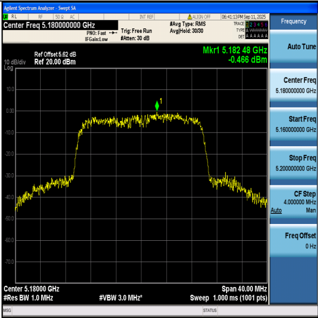
11AX20-Ant1+2-5180-PASS
