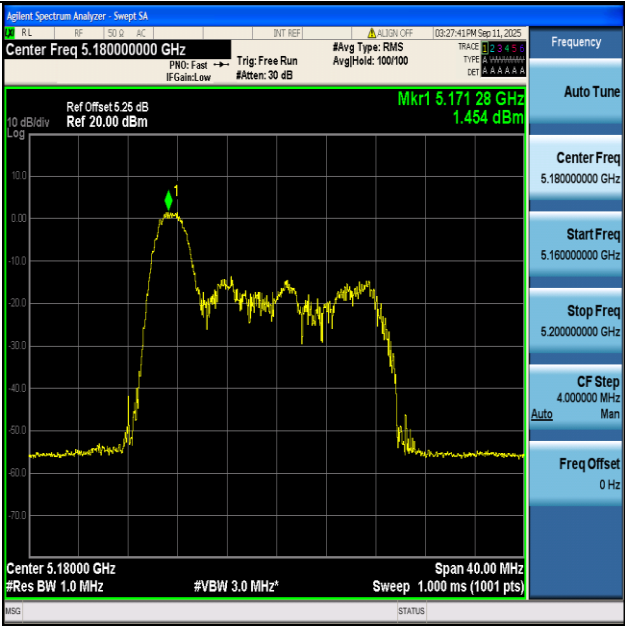
11AX20-Ant1+2-5180-26Tone-RU0-PASS
