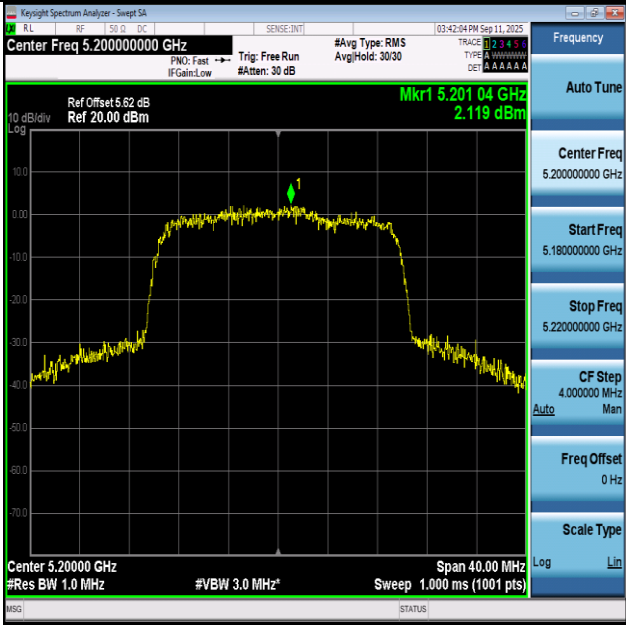
11AX20-Ant1+2-5200-PASS
