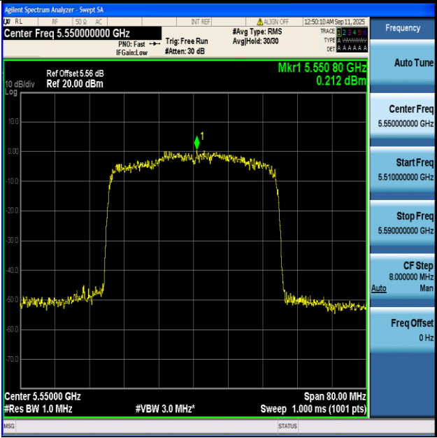
11AX40-Ant1+2-5550-PASS
