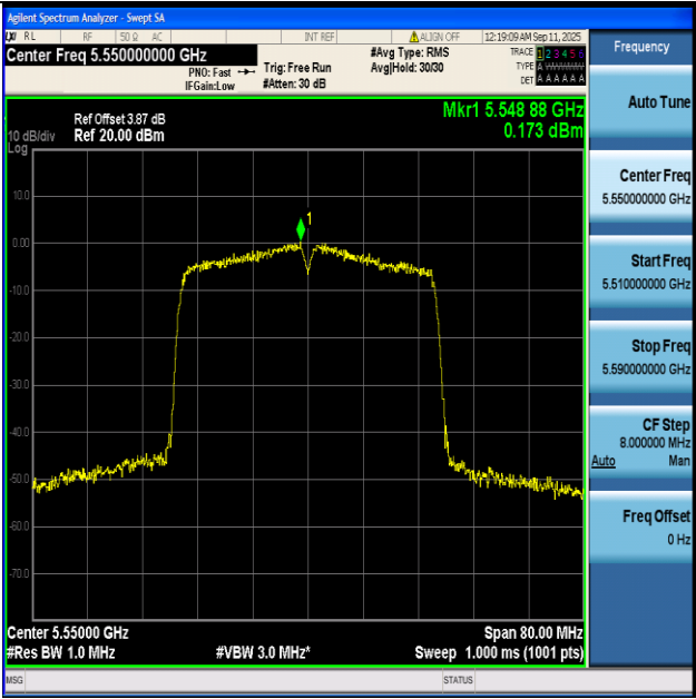
11AC40-Ant1+2-5550-PASS
