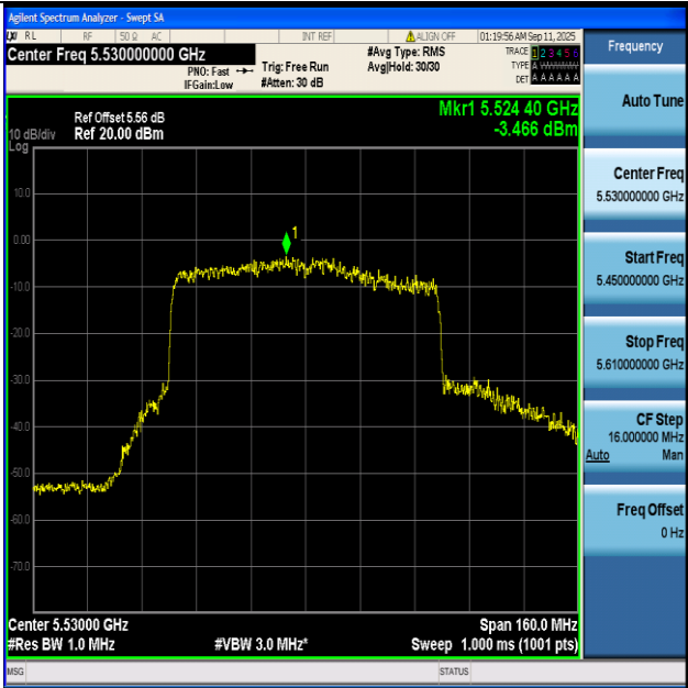
11BE80-Ant1+2-5530-PASS
