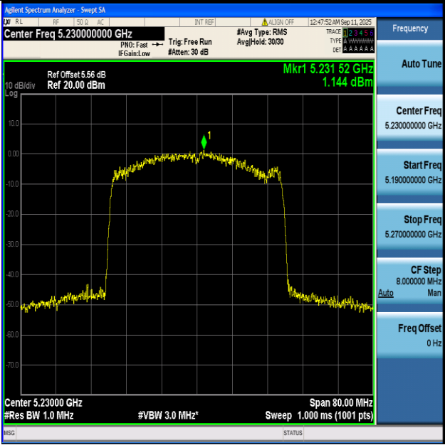
11AX40-Ant1+2-5230-PASS
