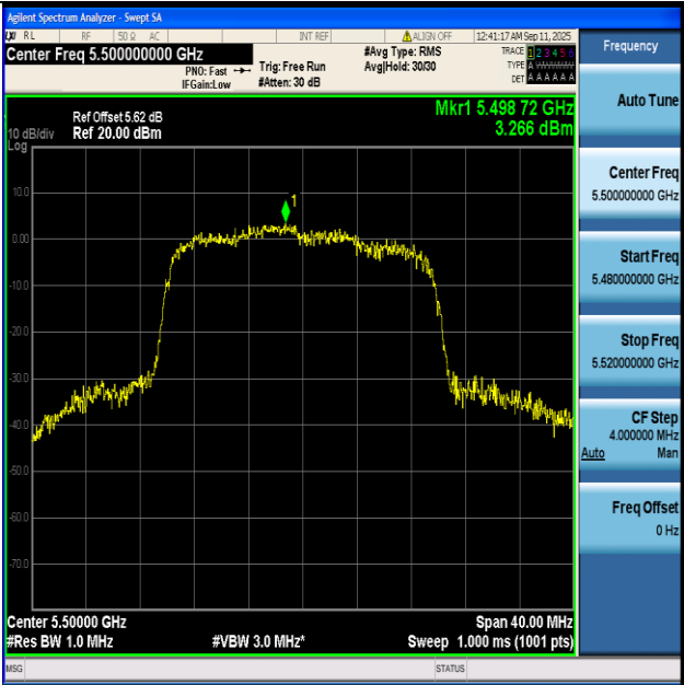
11AX20-Ant1+2-5500-PASS
