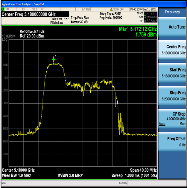
11AX20-Ant1+2-5180-52Tone-RU37-PASS
