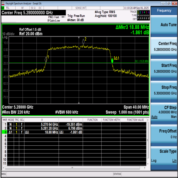
11AC20SISO-Ant1-5280
