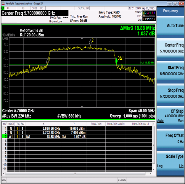
11AC20SISO-Ant1-5700
