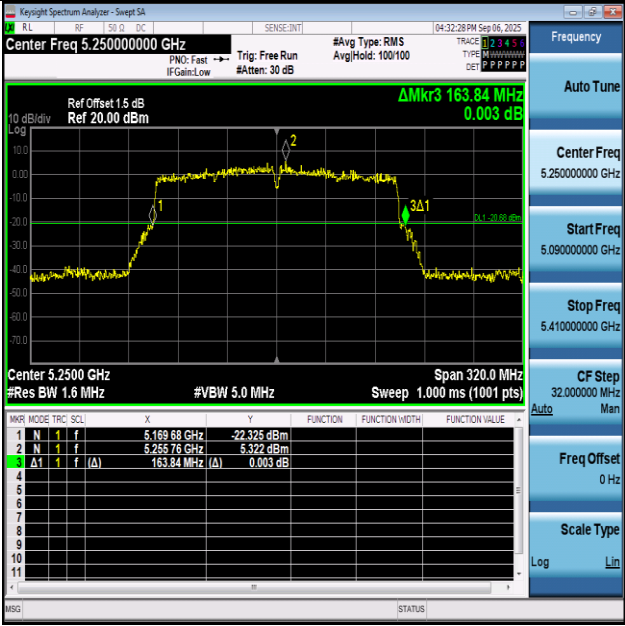
11AC160SISO-Ant1-5250
