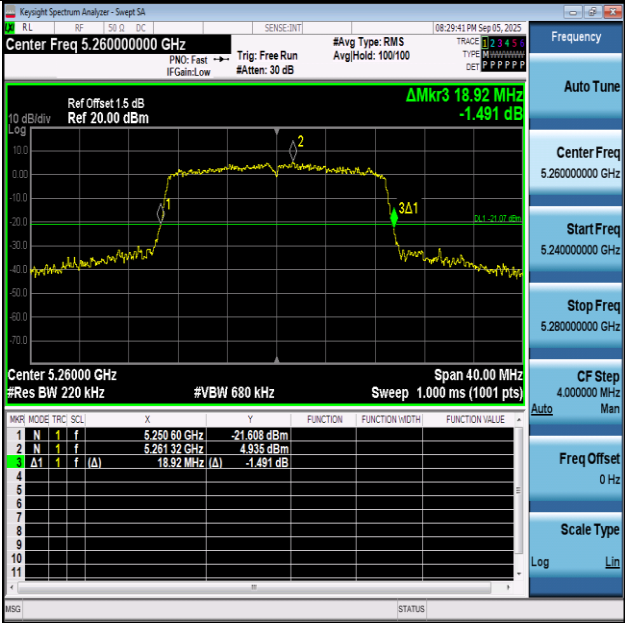
11N20SISO-Ant1-5260
