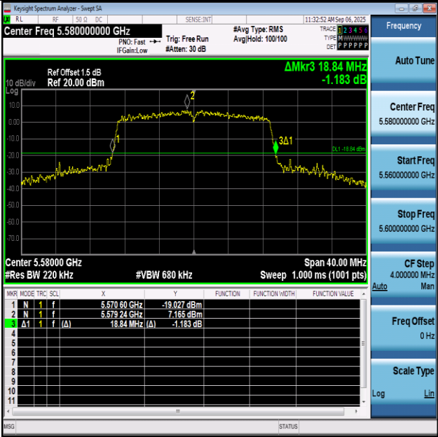
11AC20SISO-Ant1-5580
