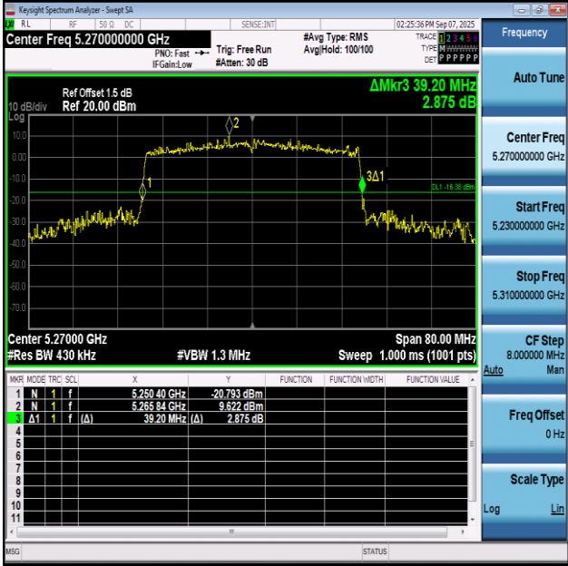
11BE40SISO-Ant1-5270
