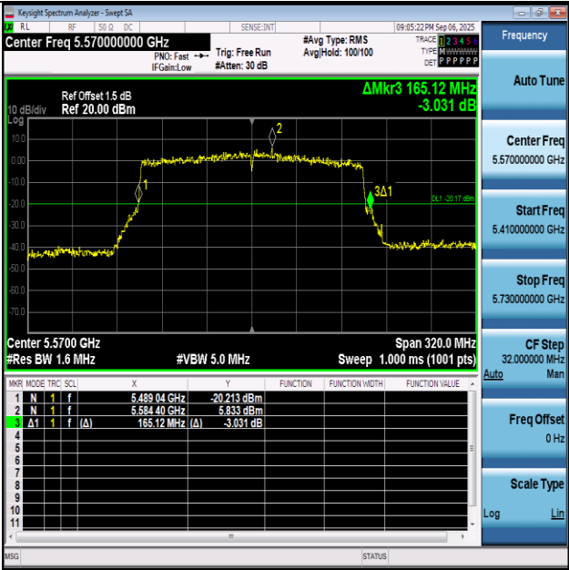
11AX160SISO-Ant1-5570
