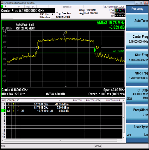
11BE20SISO-Ant1-5180
