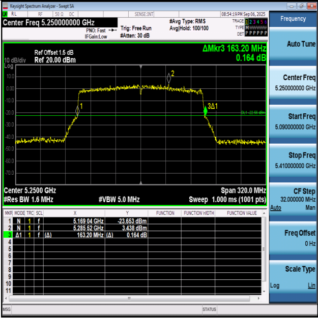
11AX160SISO-Ant1-5250
