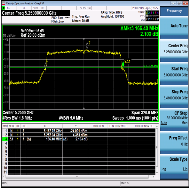
11BE160SISO-Ant1-5250
