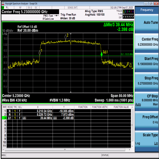
11BE40SISO-Ant1-5230
