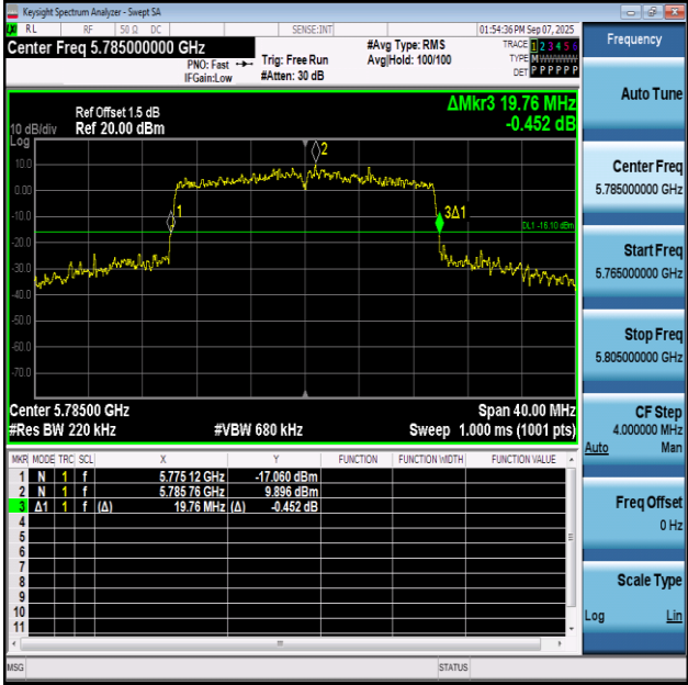
11BE20SISO-Ant1-5785
