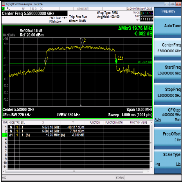
11BE20SISO-Ant1-5580
