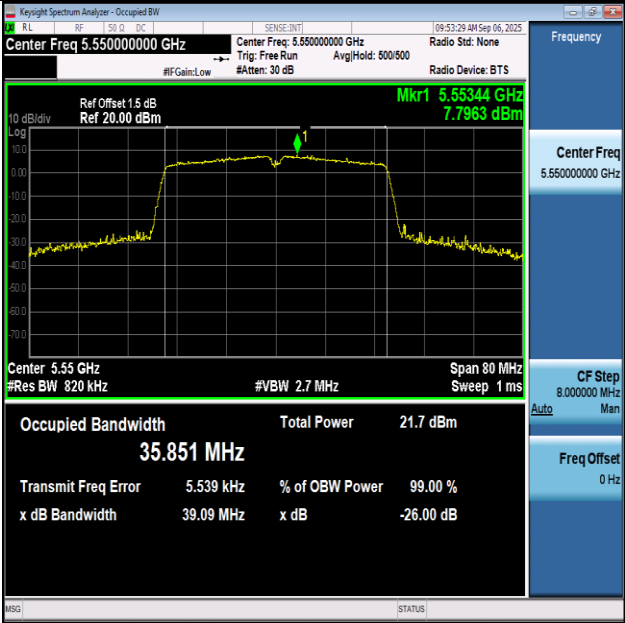
11N40SISO-Ant1-5550
