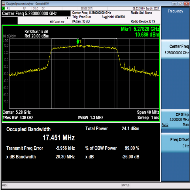
11AC20SISO-Ant1-5280
