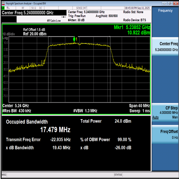
11AC20SISO-Ant1-5240
