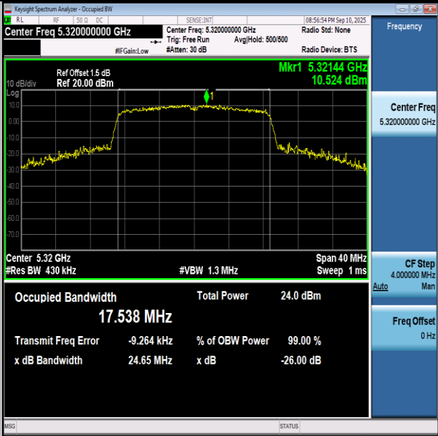
11AC20SISO-Ant1-5320
