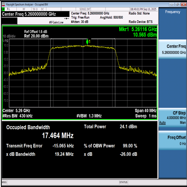
11AC20SISO-Ant1-5260
