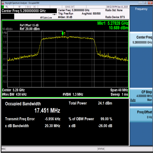
11AC20SISO-Ant1-5280
