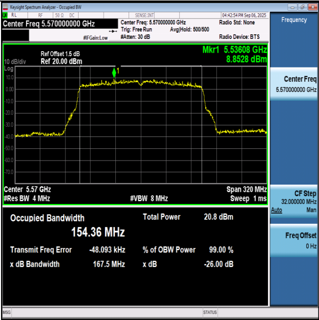
11AC160SISO-Ant1-5570
