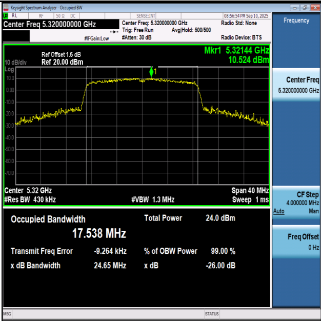
11AC20SISO-Ant1-5320
